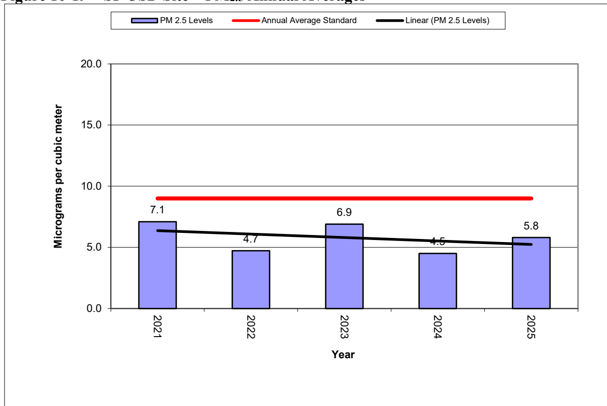
Figure 10-19 – SF USD Site – PM 2.5 Annual Averages
