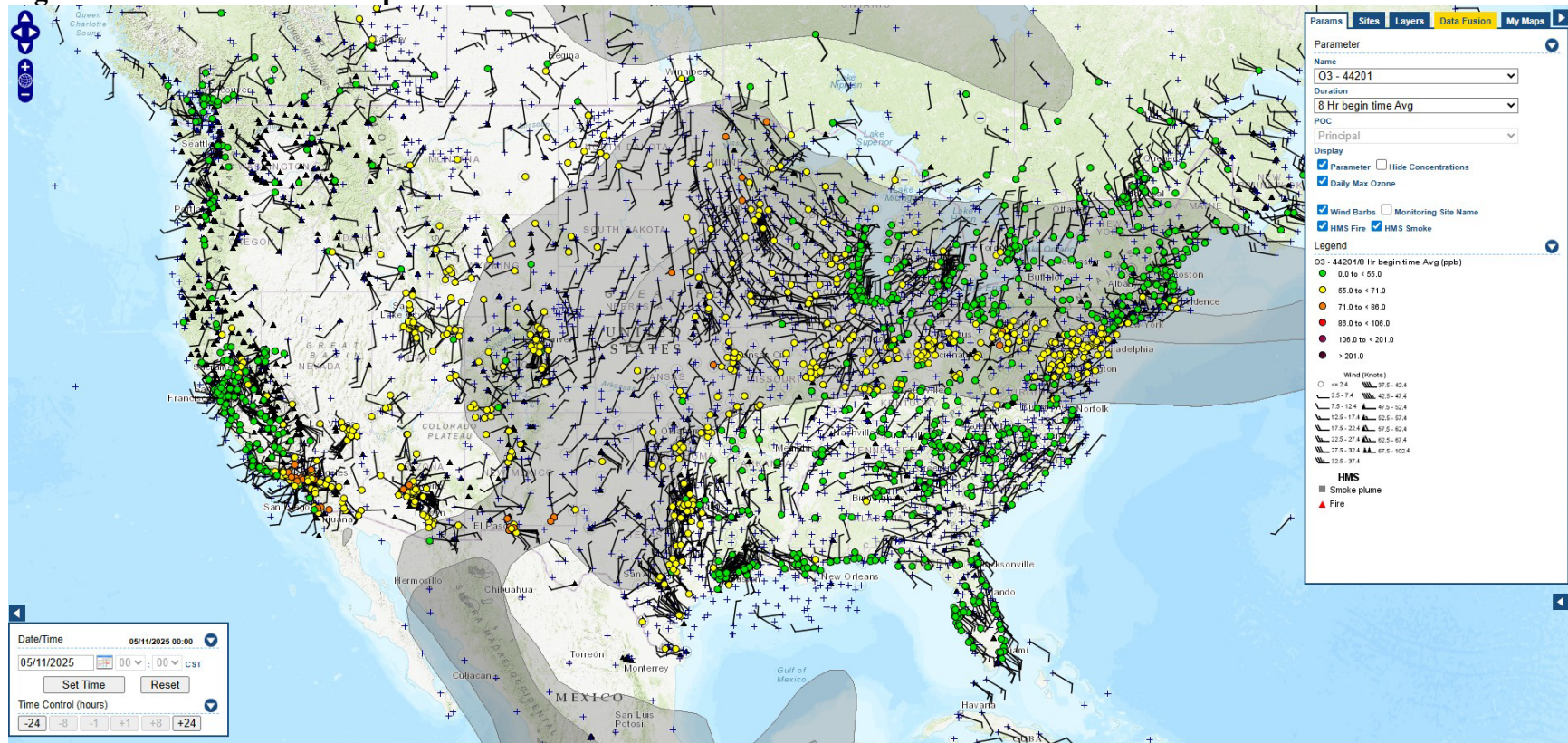
Figure C-6 - AirNow Tech Map for 05/11/25
