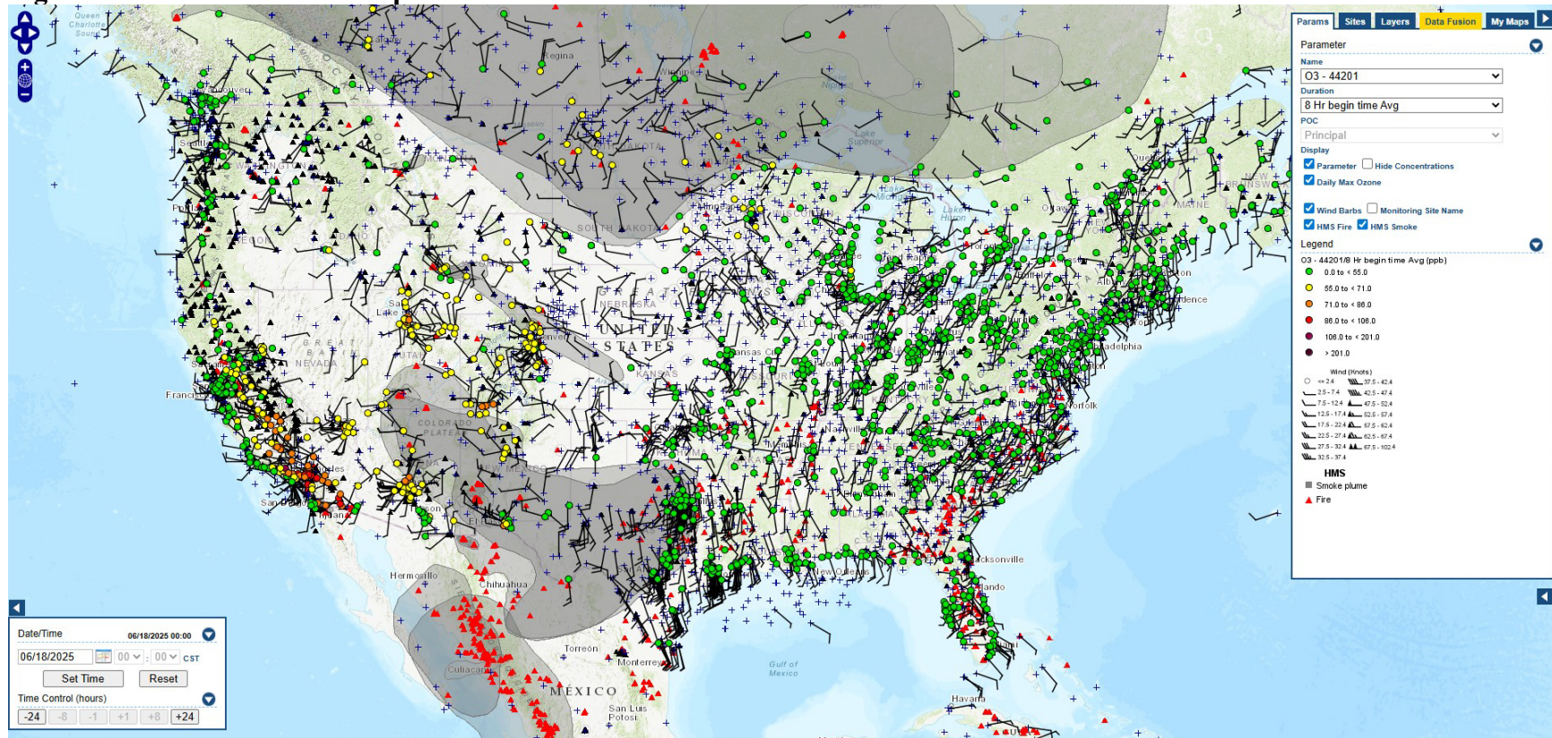
Figure C-20 - AirNow Tech Map for 06/18/25
