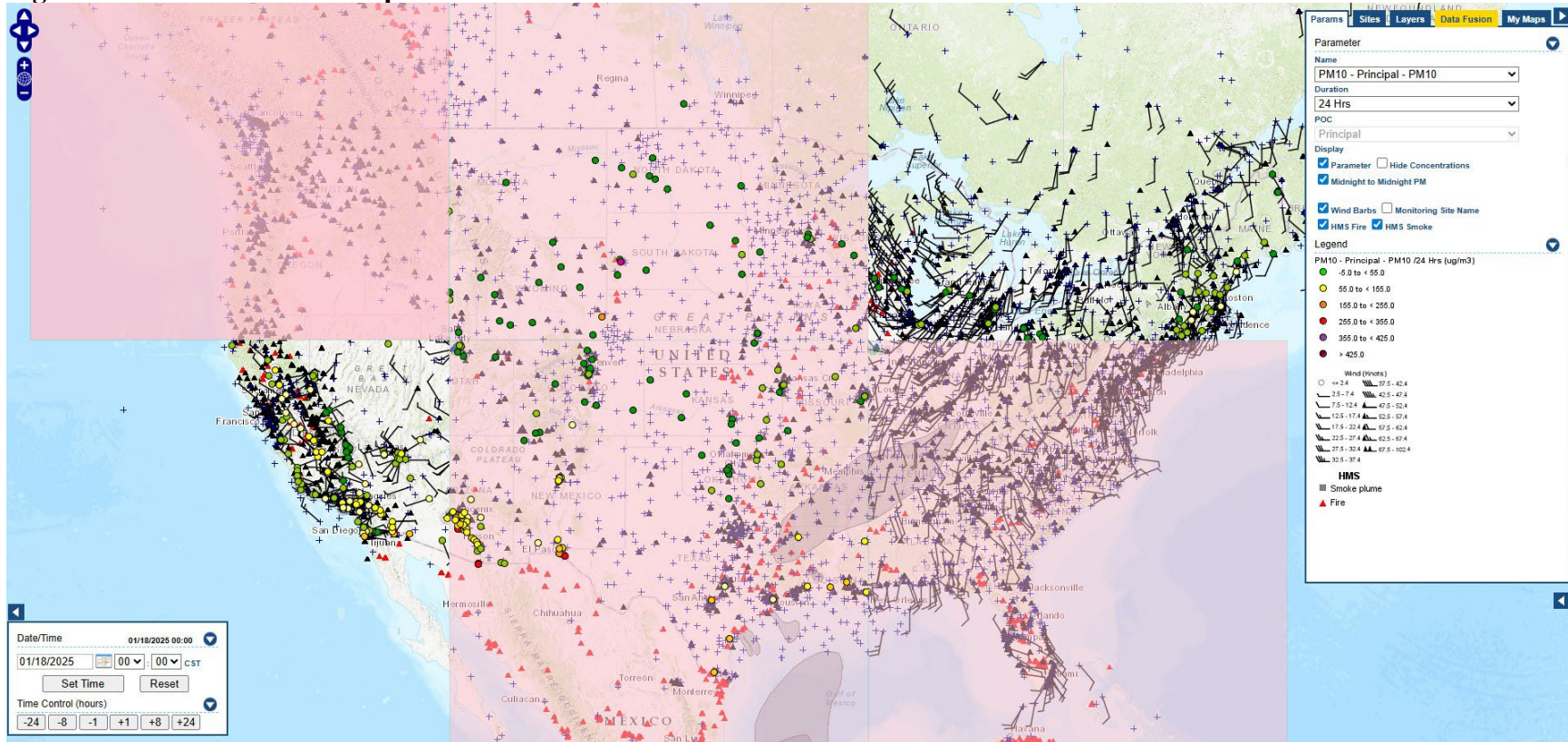
Figure B-4 – AirNow Tech Map for 01/18/25
