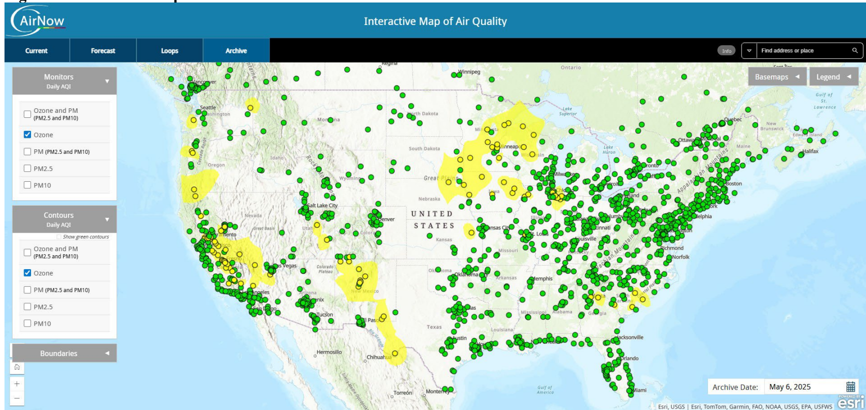
Figure C-1 - AirNow Map for 05/06/25
