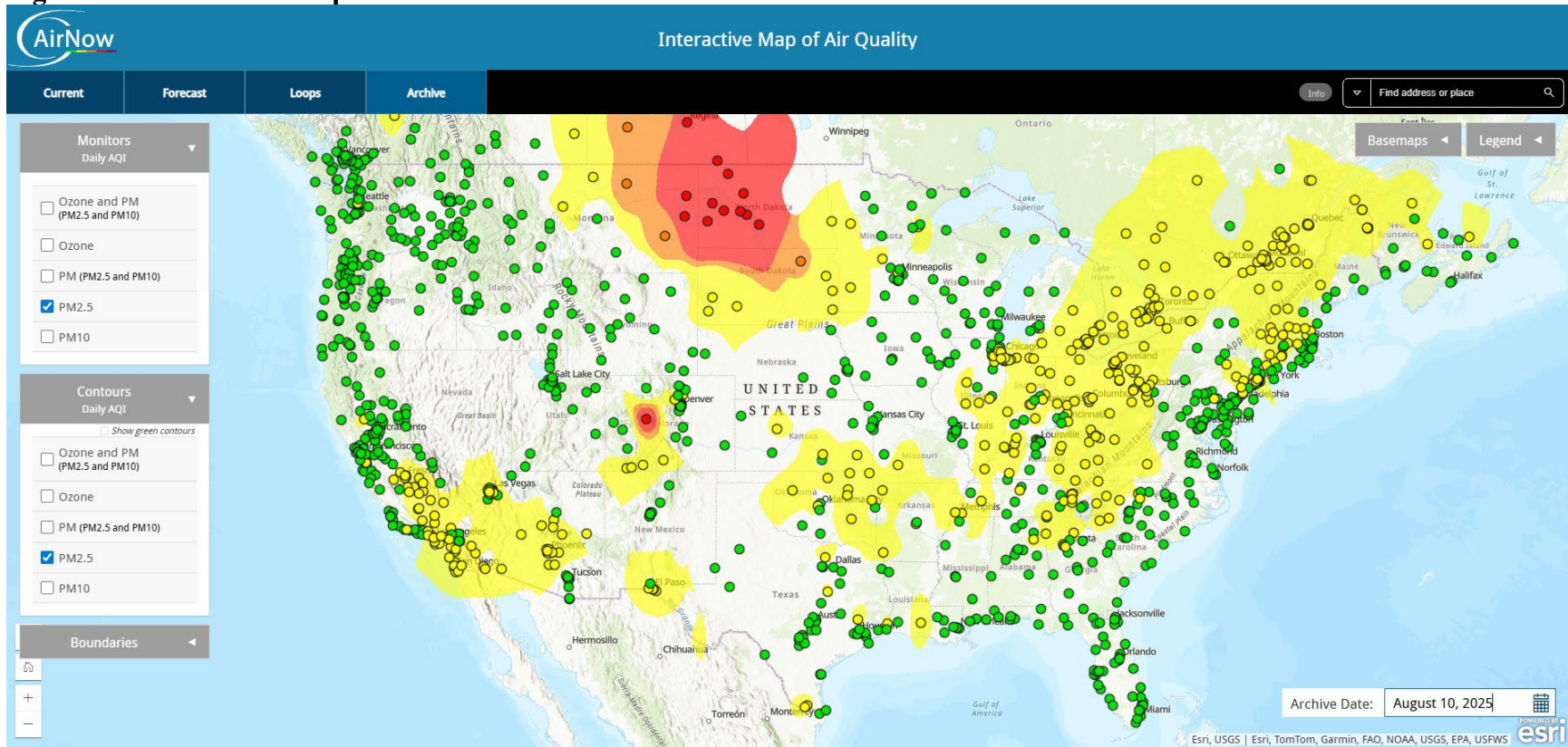
Figure A-17 – AirNow Map for 08/10/25
