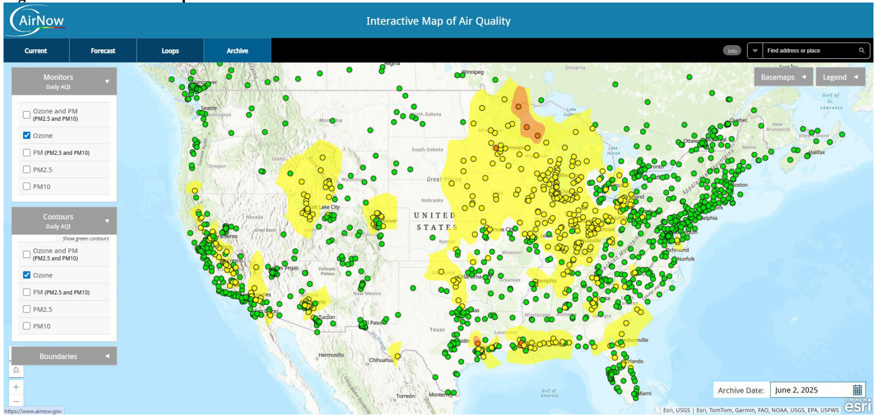
Figure C-15 - AirNow Map for 06/02/25
