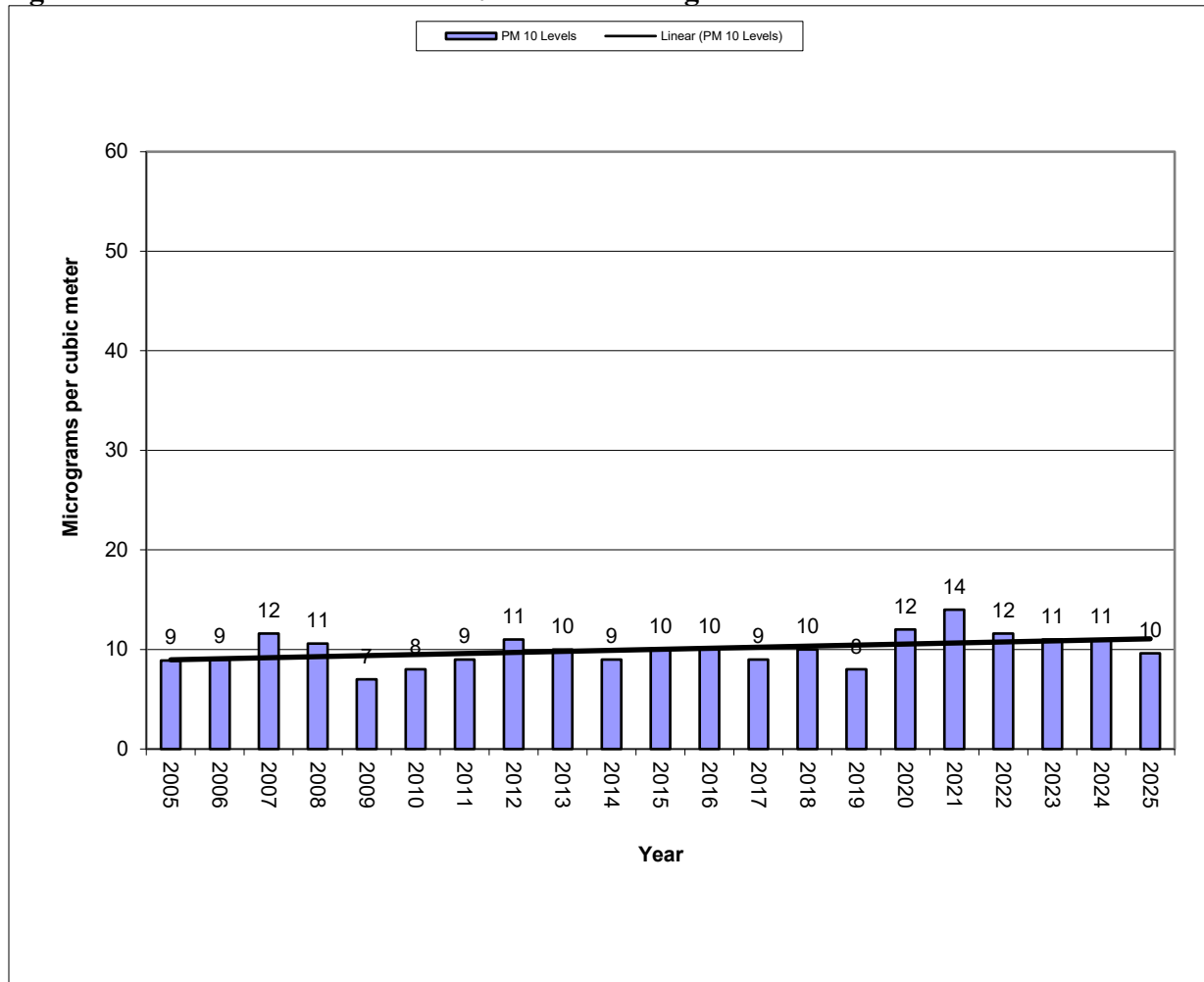
Figure 10-10 – Badlands Site – PM 10 Annual Averages
