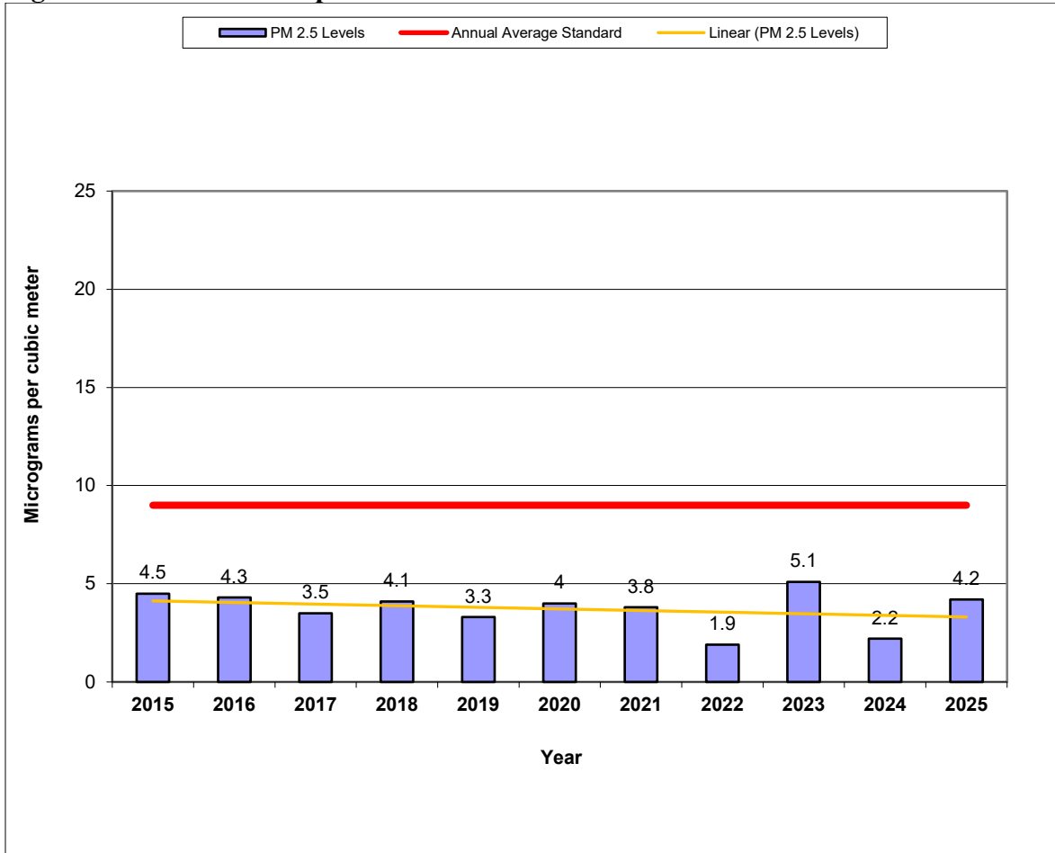
Figure 10-39 – Pierre Airport Site – Annual PM 2.5 Concentrations
