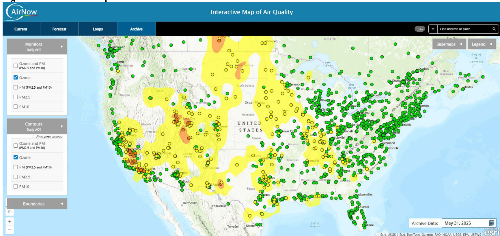
Figure C-11 - AirNow Map for 05/31/25
