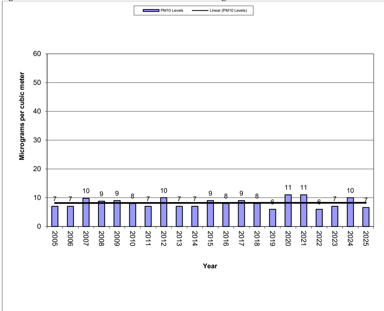
Figure 10-14 - Wind Cave Site – PM 10 Annual Averages
