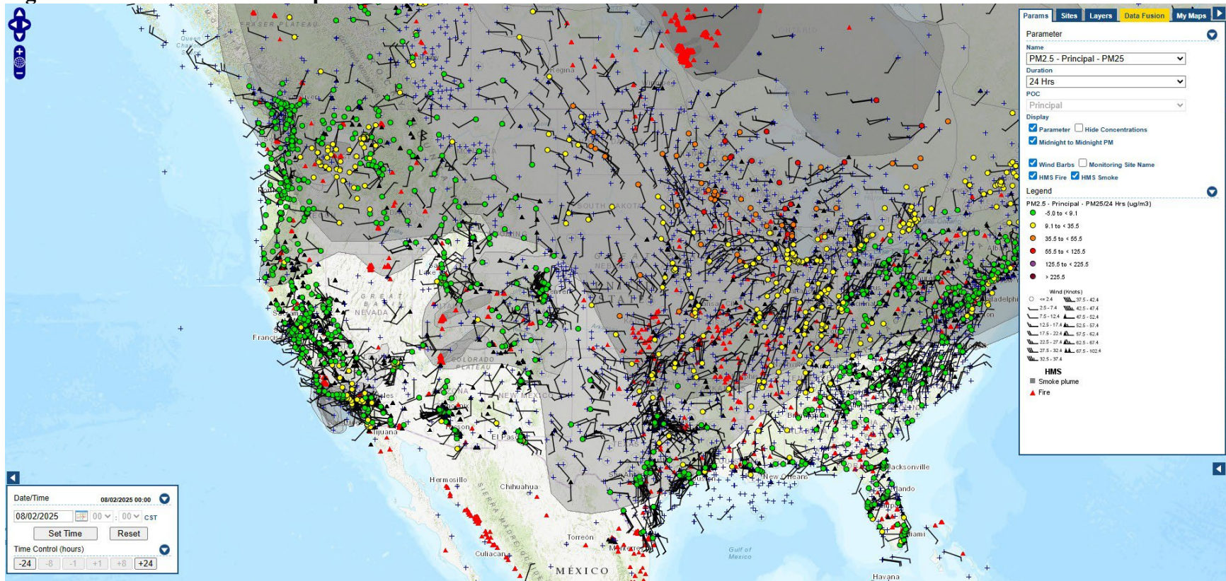
Figure A-16 – AirNow Tech Map for 08/02/25
