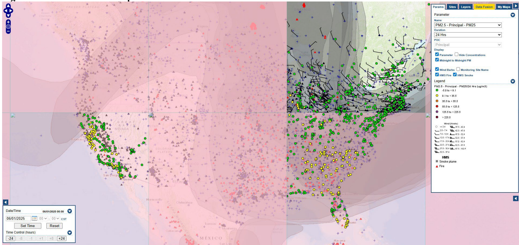
Figure A-4 – AirNow Tech Map for 06/01/25
