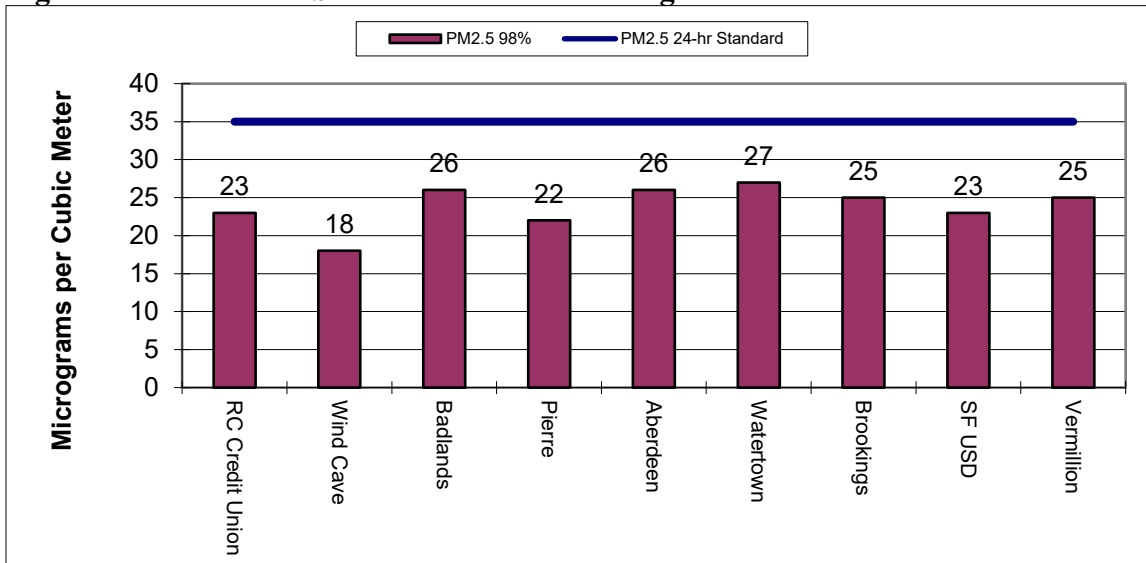
Figure 9-1 – 2025 PM 2.5 Statewide 24-Hour Design Values
