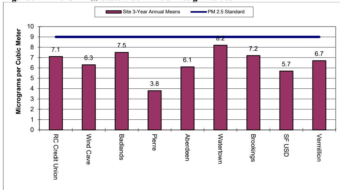
Figure 9-2 – 2025 PM 2.5 Statewide Annual Design Values
