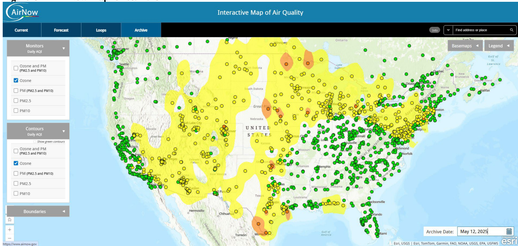
Figure C-7 - AirNow Map for 05/12/25
