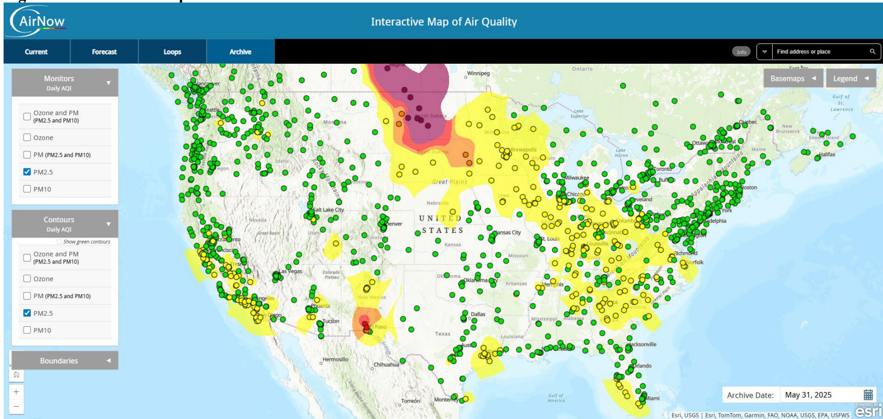
Figure A-1 – AirNow Map for 05/31/25
