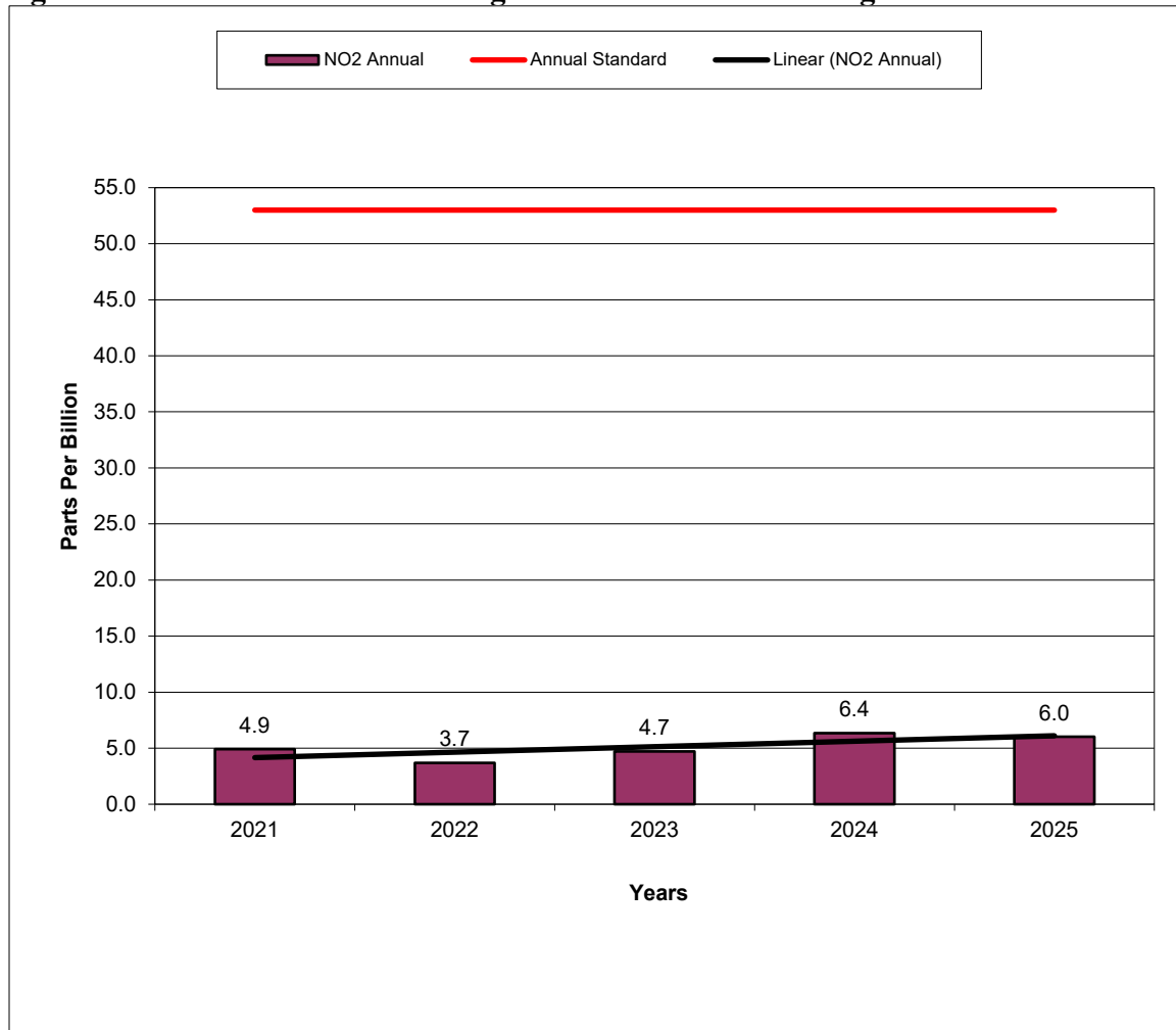
Figure 10-22 – SF USD Site – Nitrogen Dioxide Annual Averages
