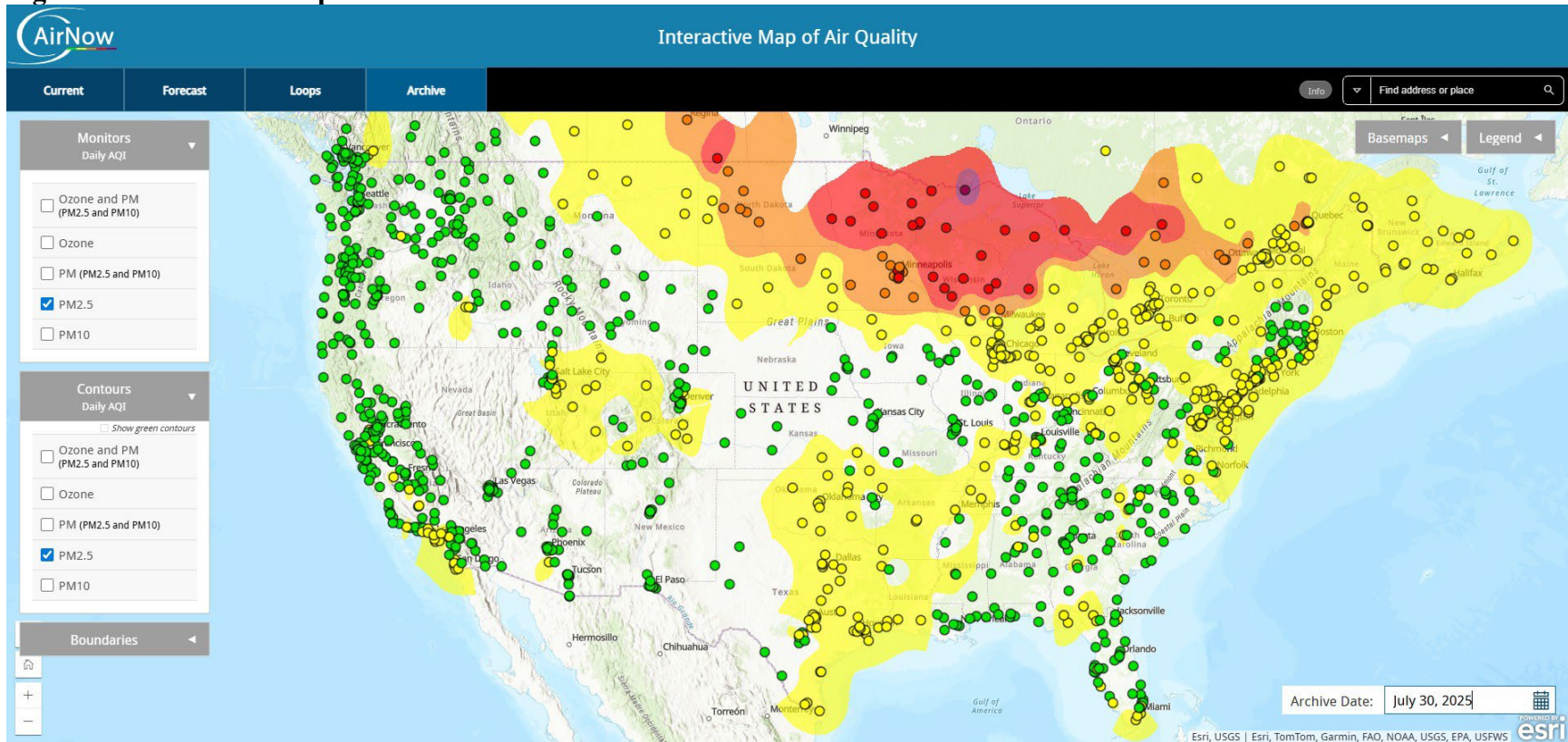
Figure A-9 – AirNow Map for 07/30/25
