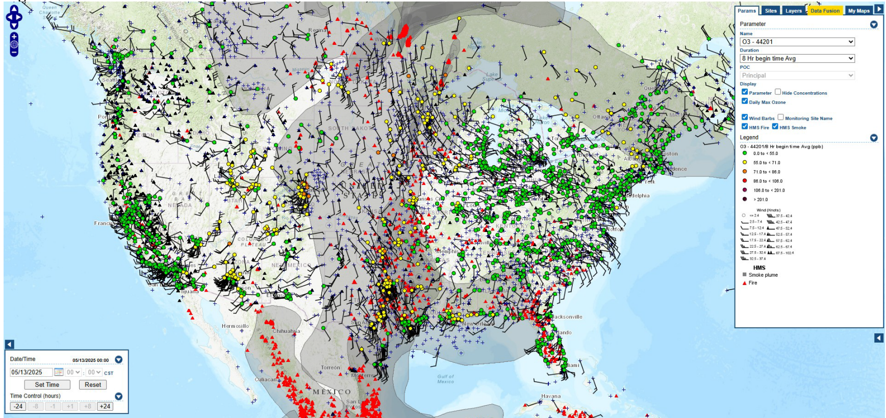
Figure C-10 - AirNow Tech Map for 05/13/25
