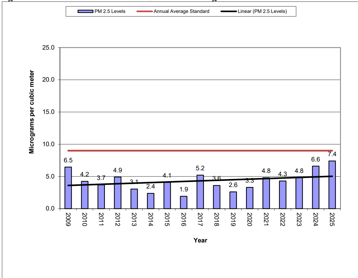
Figure 10-15 - Wind Cave Site – PM 2.5 Annual Averages
