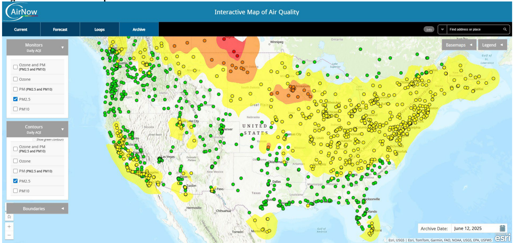
Figure A-5 – AirNow Map for 06/12/25
