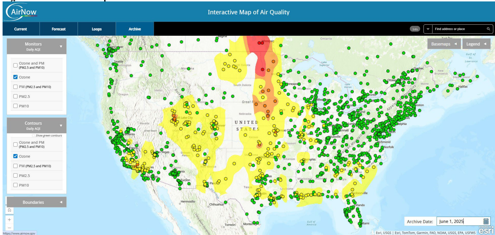
Figure C-13 - AirNow Map for 06/01/25
