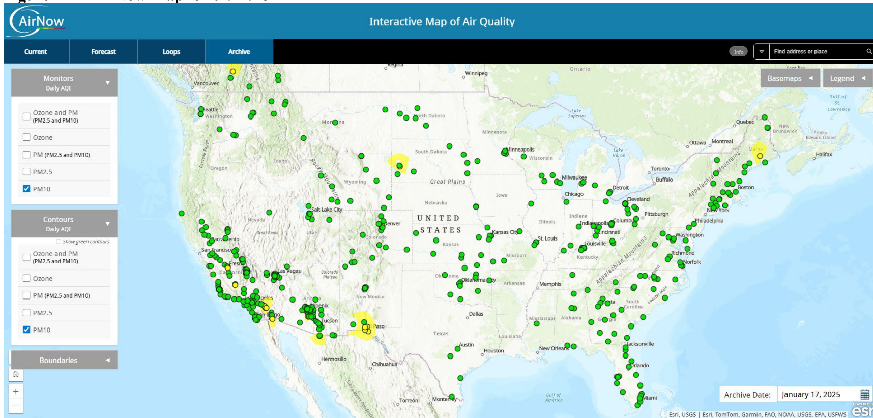
Figure B-1 - AirNow Map for 01/17/25
