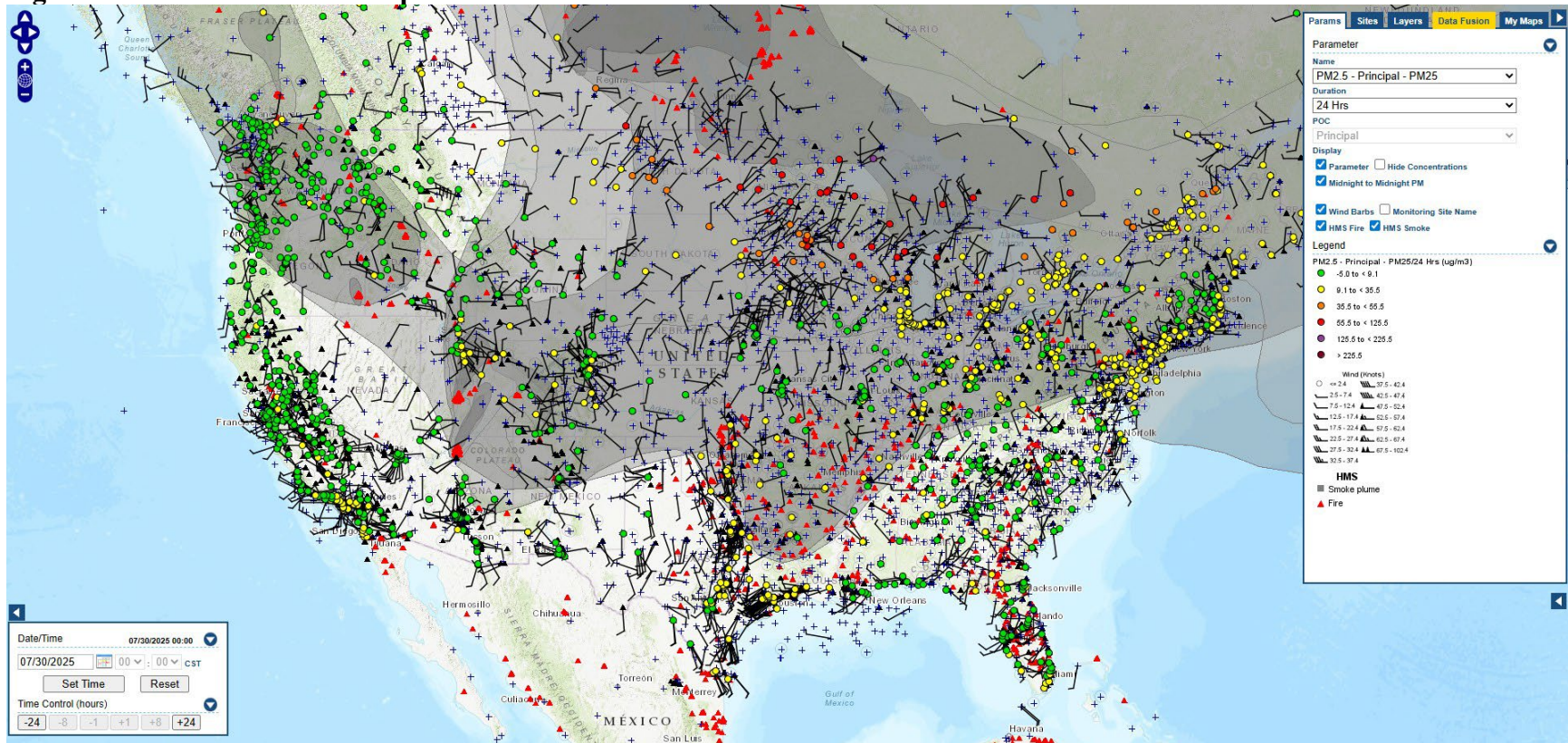
Figure A-10 – AirNow Tech Map for 07/30/25
