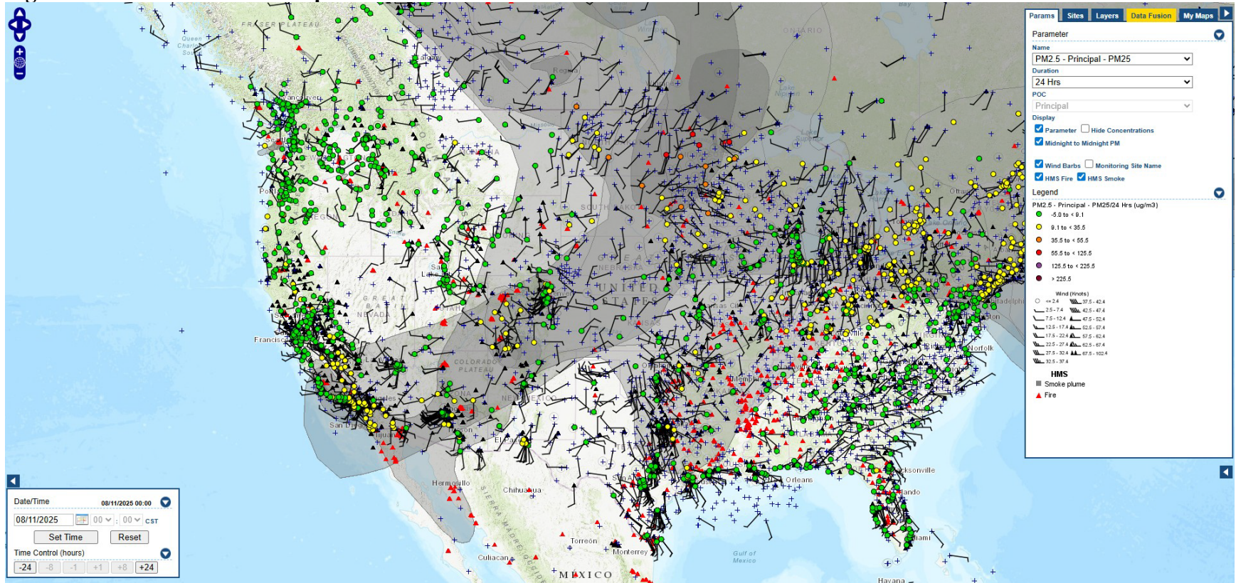
Figure A-20 – AirNow Tech Map for 08/11/25
