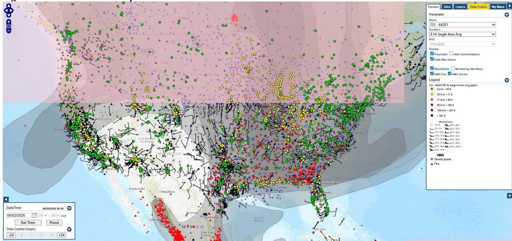
Figure C-16 - AirNow Tech Map for 06/02/25
