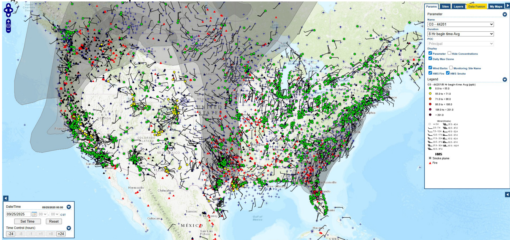
Figure C-28 - AirNow Tech Map for 09/25/25
