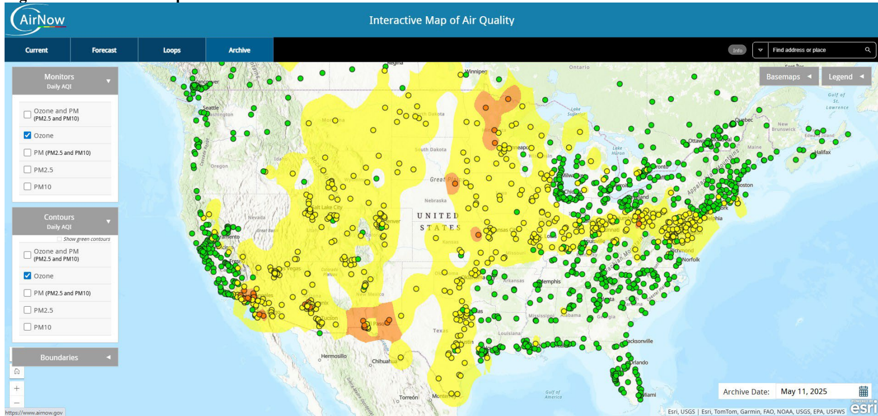
Figure C-5 - AirNow Map for 05/11/25
