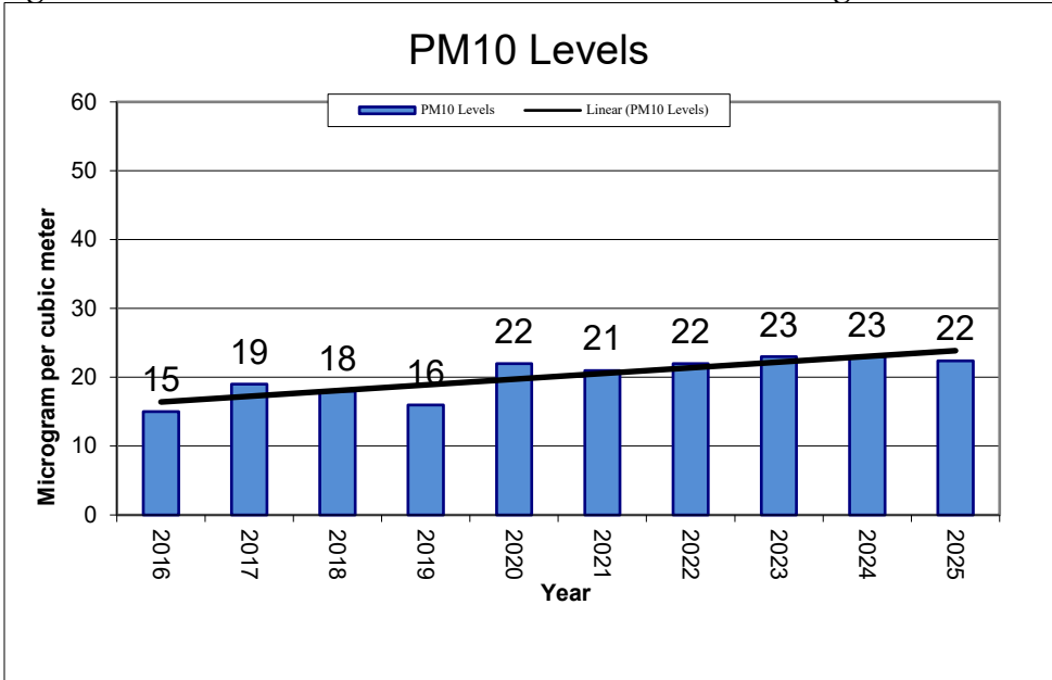
Figure 10-28 –Research Farm Site – PM 10 Annual Averages
