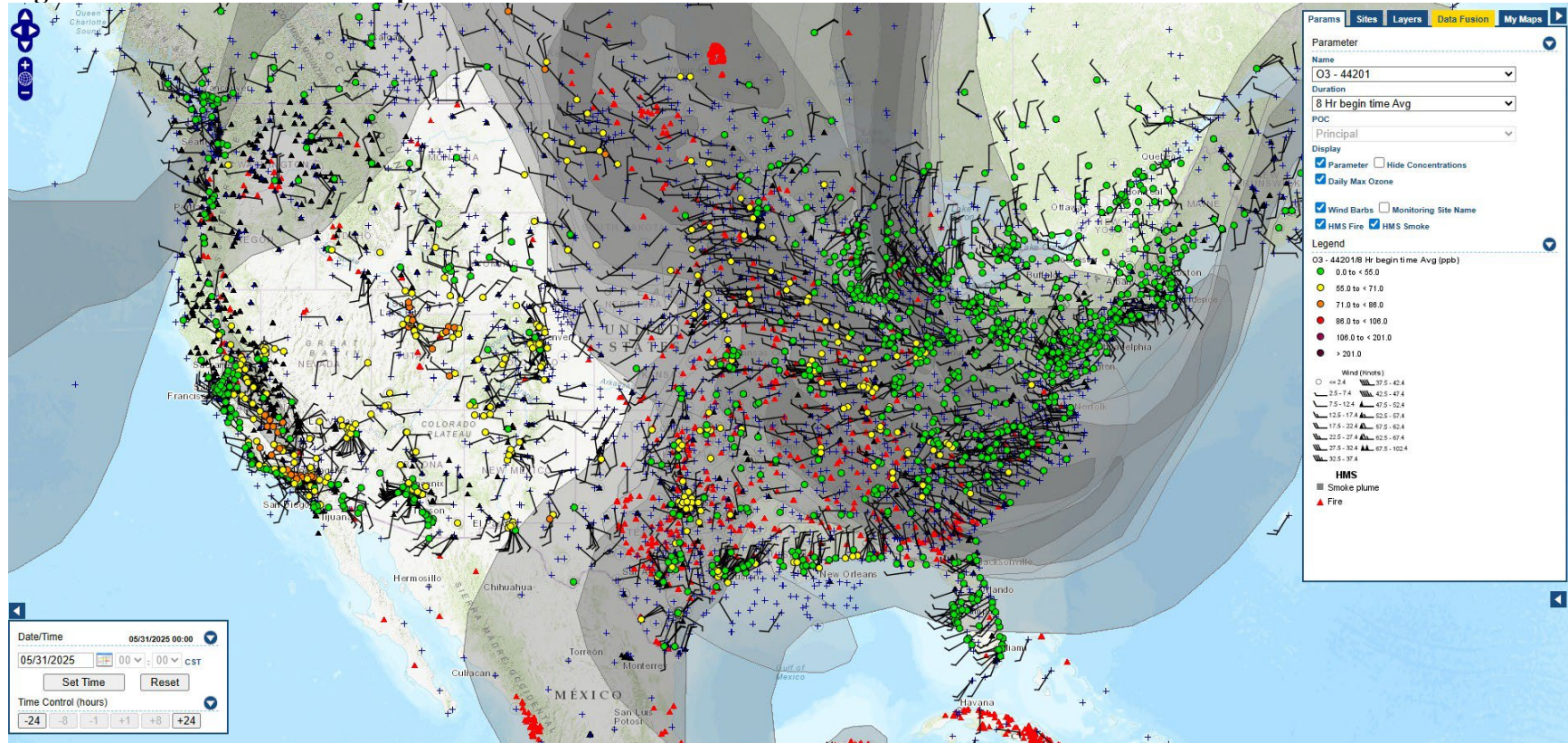
Figure C-12 - AirNow Tech Map for 05/31/25
