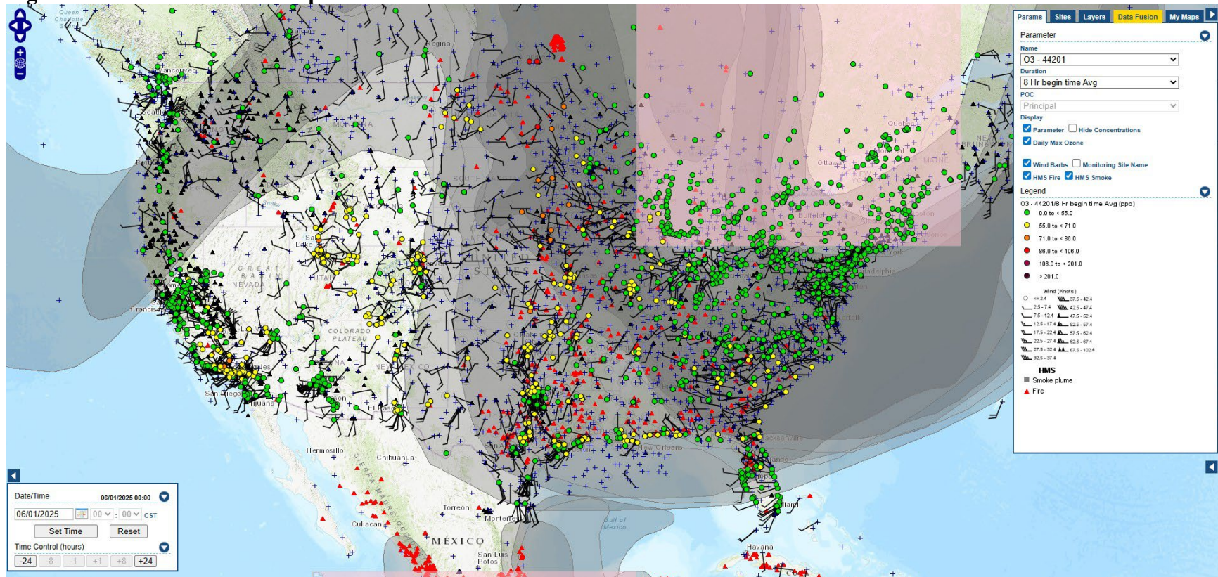
Figure C-14 - AirNow Tech Map for 06/01/25
