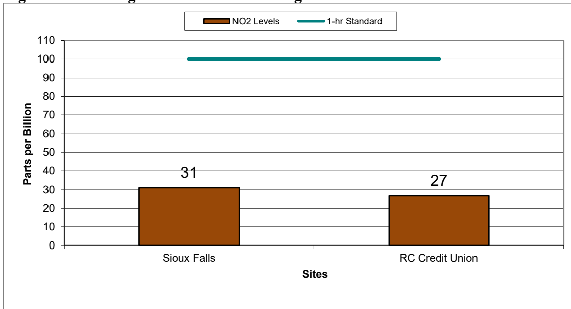
Figure 9-5 – Nitrogen Dioxide 1-hour Design Values 2025
