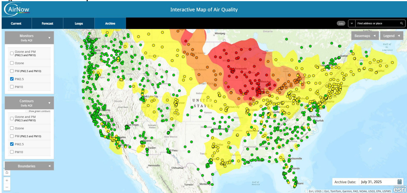
Figure A-11 – AirNow Map for 07/31/25
