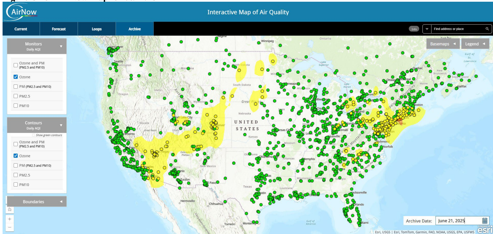
Figure C-25 - AirNow Map for 06/21/25
