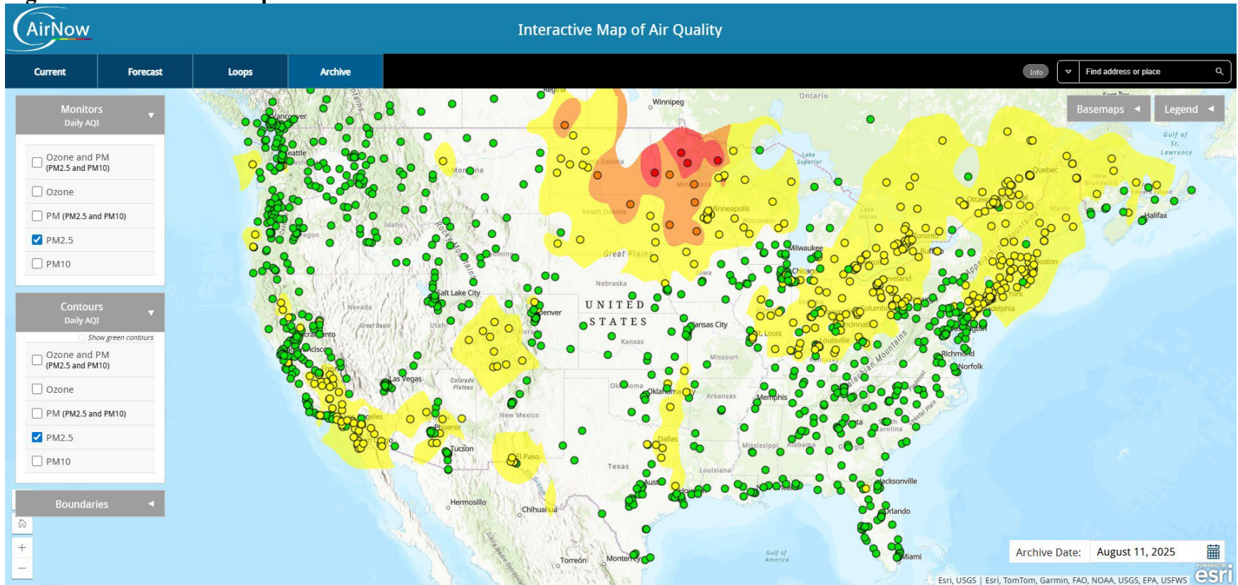
Figure A-19 – AirNow Map for 08/11/25
