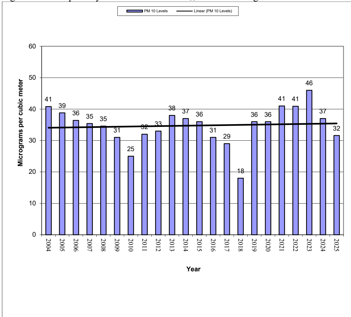
Figure 10-2 – Rapid City Credit Union Site PM 10 Annual Averages
