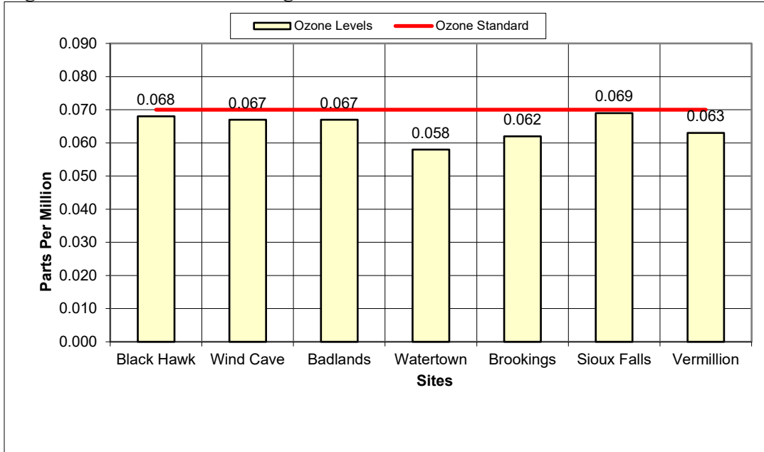
Figure 9-3– 2025 Ozone Design Values Statewide
