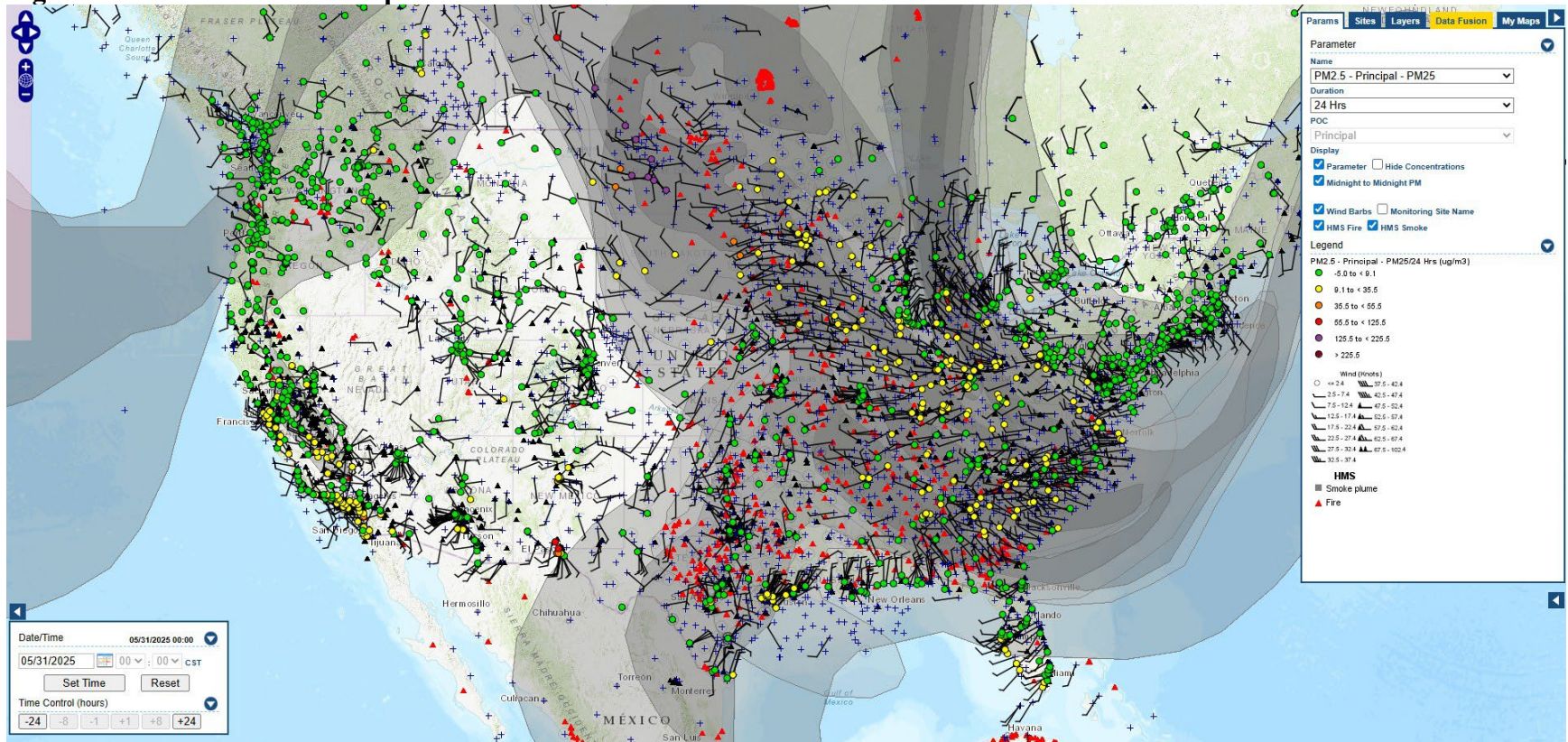
Figure A-2 – AirNow Tech Map for 05/31/25
