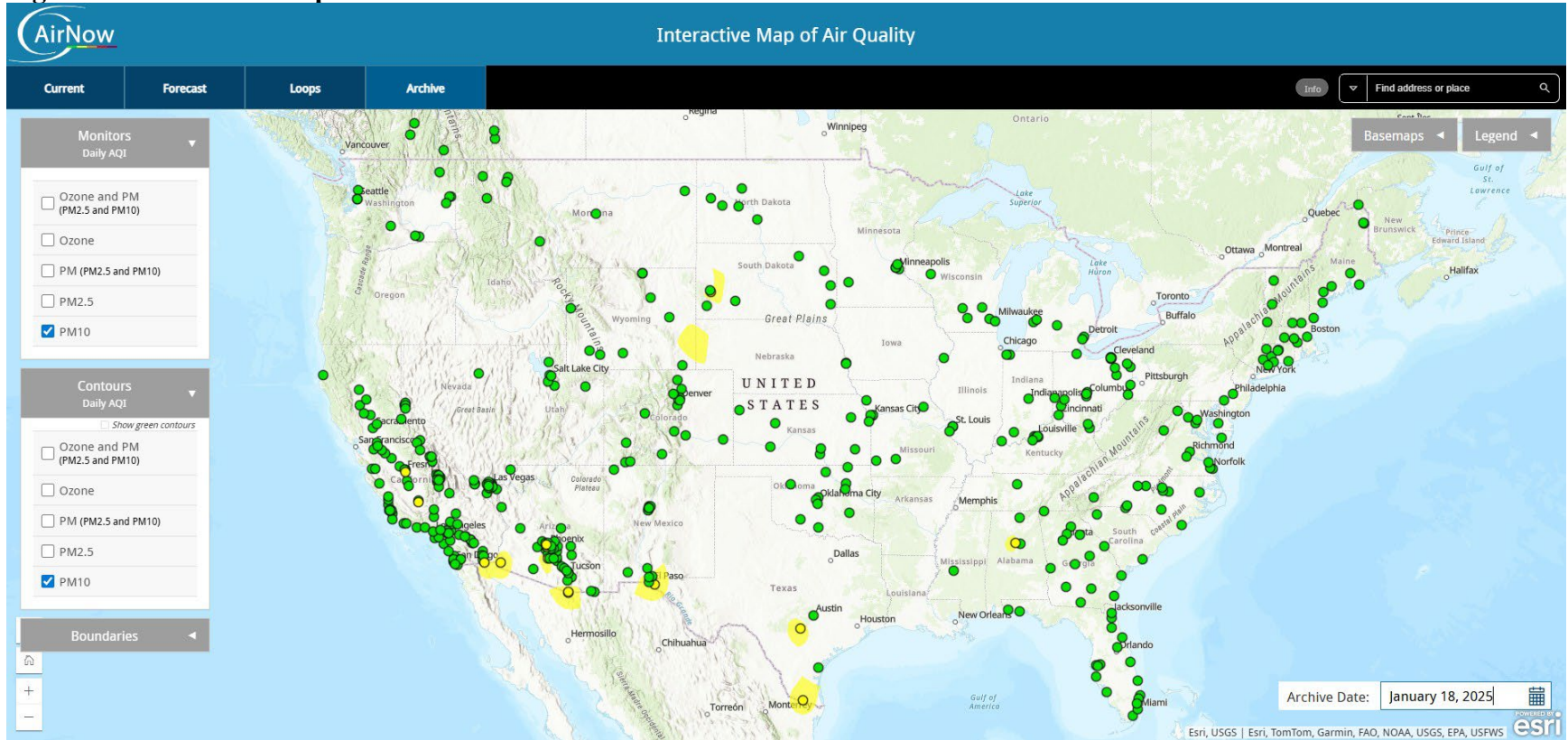
Figure B-3 – AirNow Map for 01/18/25
