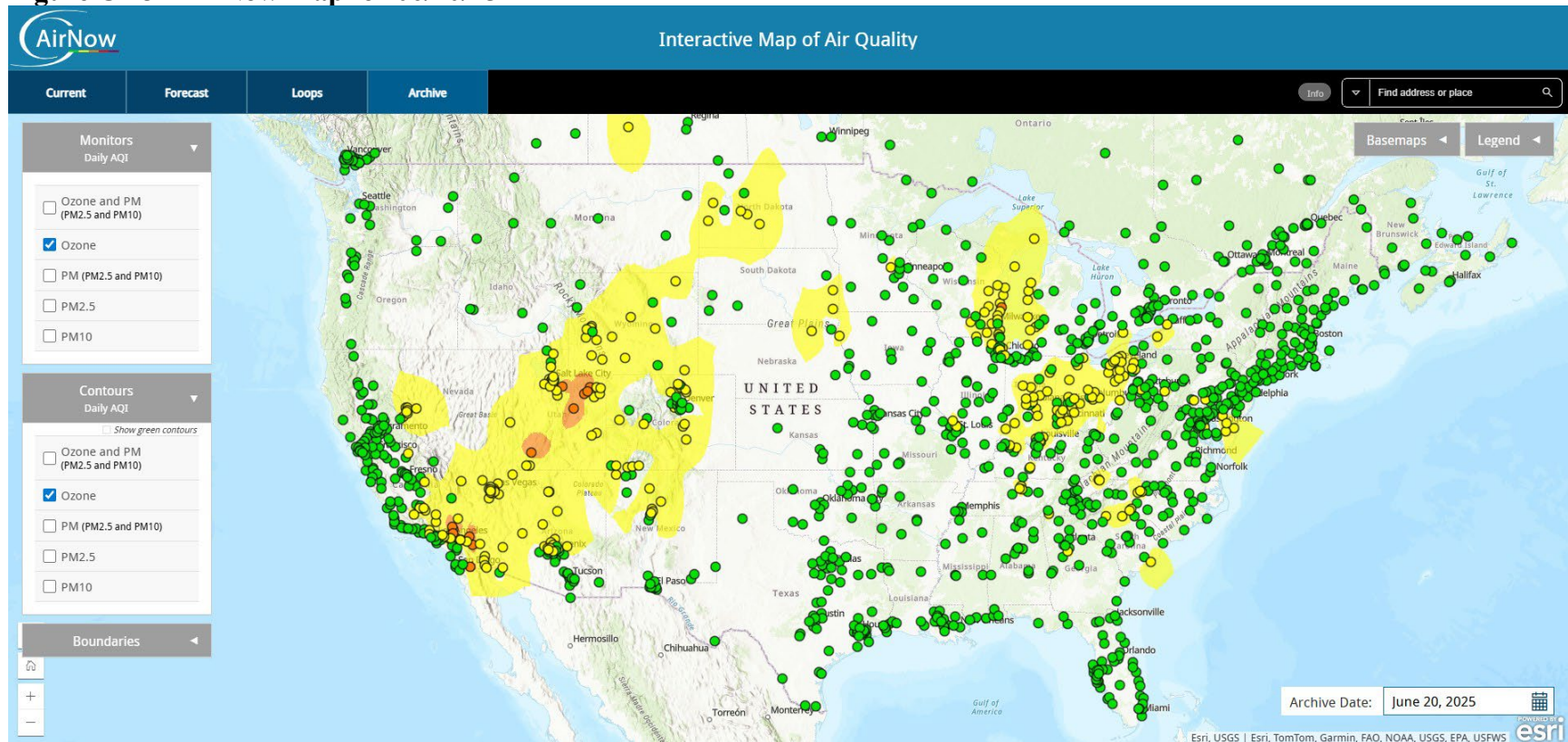
Figure C-23 - AirNow Map for 06/20/25
