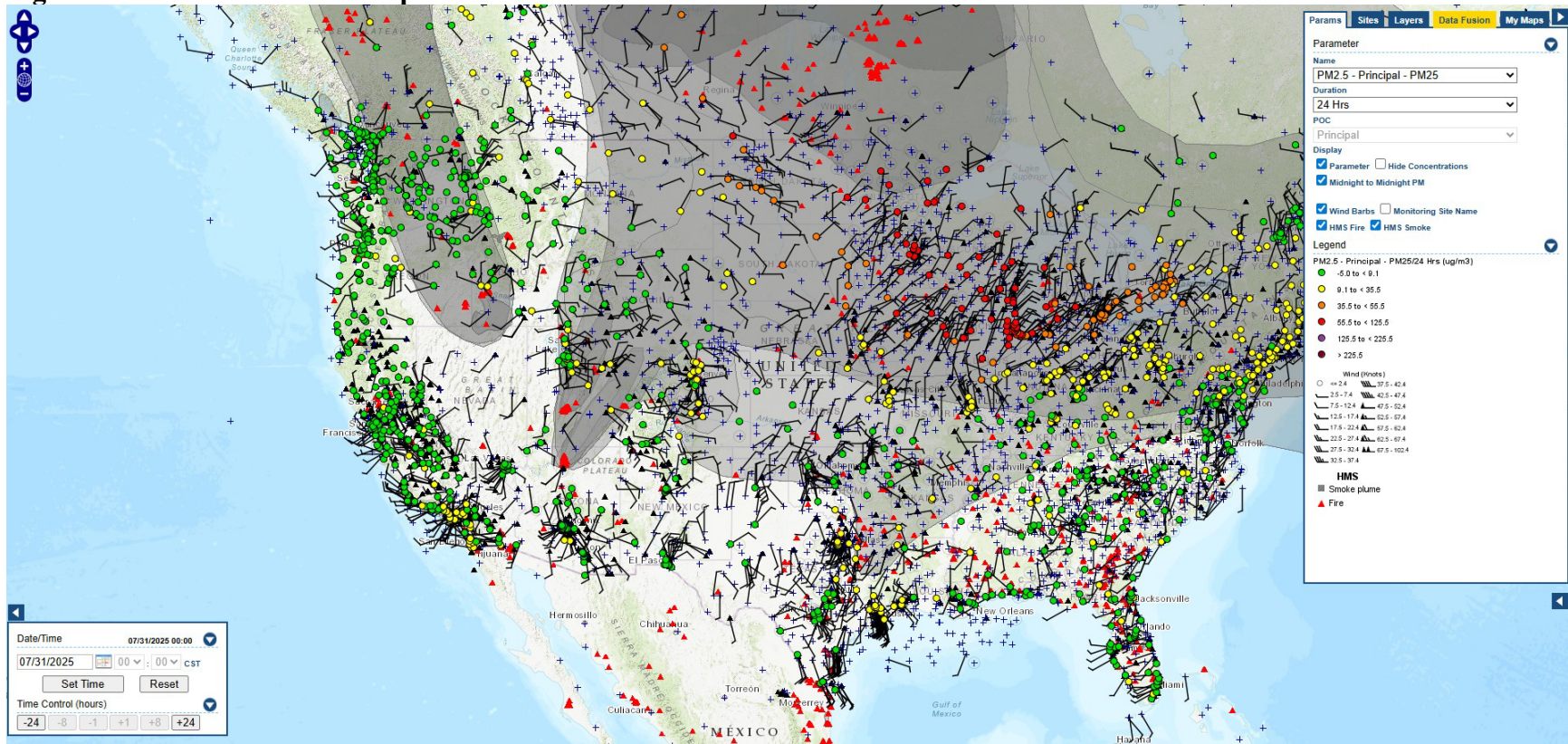
Figure A-12 – AirNow Tech Map for 07/31/25
