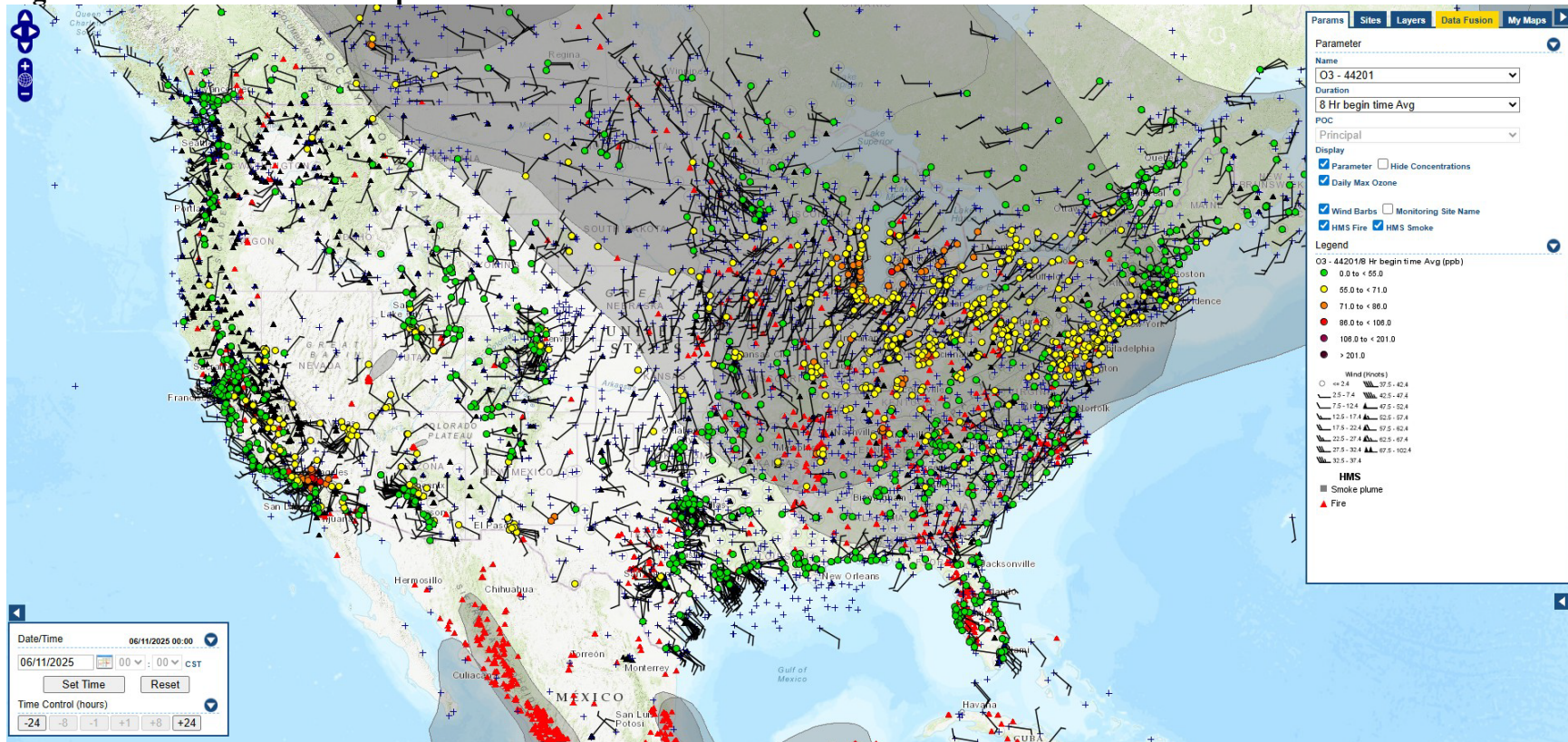
Figure C-18 - AirNow Tech Map for 06/11/25
