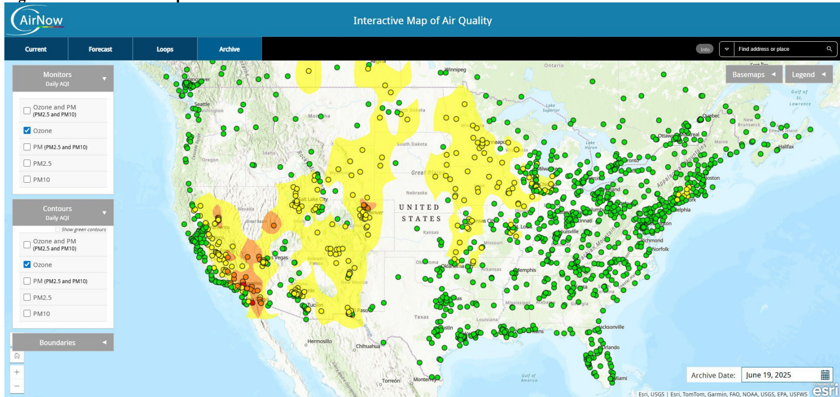
Figure C-21 - AirNow Map for 06/19/25
