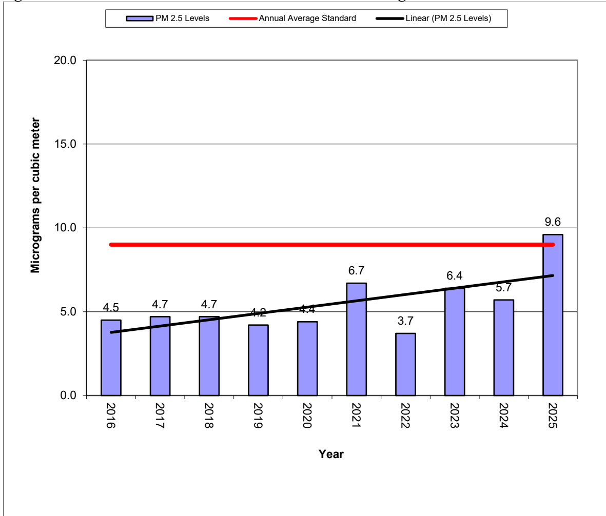
Figure 10-29 –Research Farm Site – PM 2.5 Annual Averages
