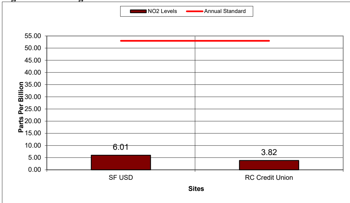
Figure 9-6 – Nitrogen Dioxide Annual Concentration 2025
