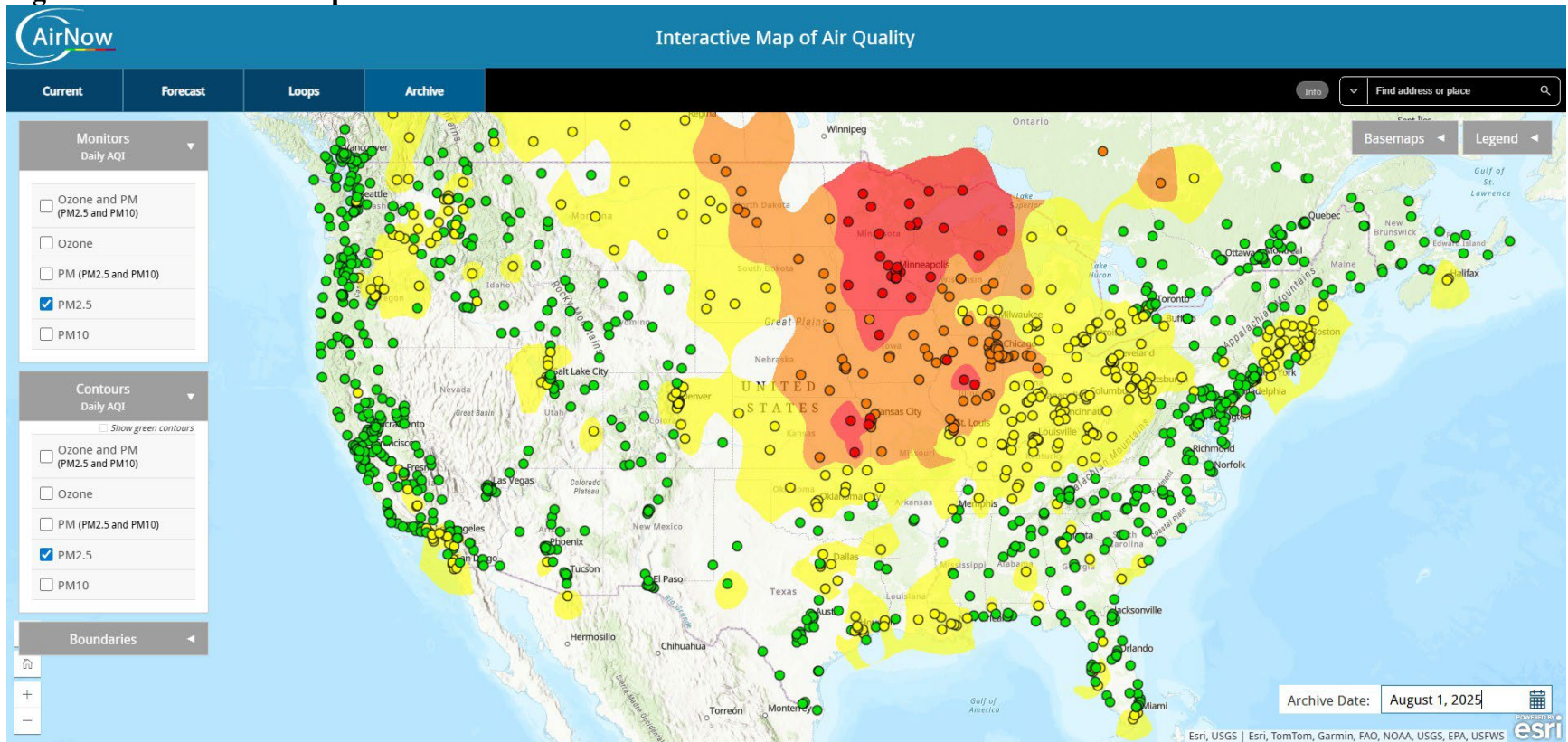
Figure A-13 – AirNow Map for 08/01/25
