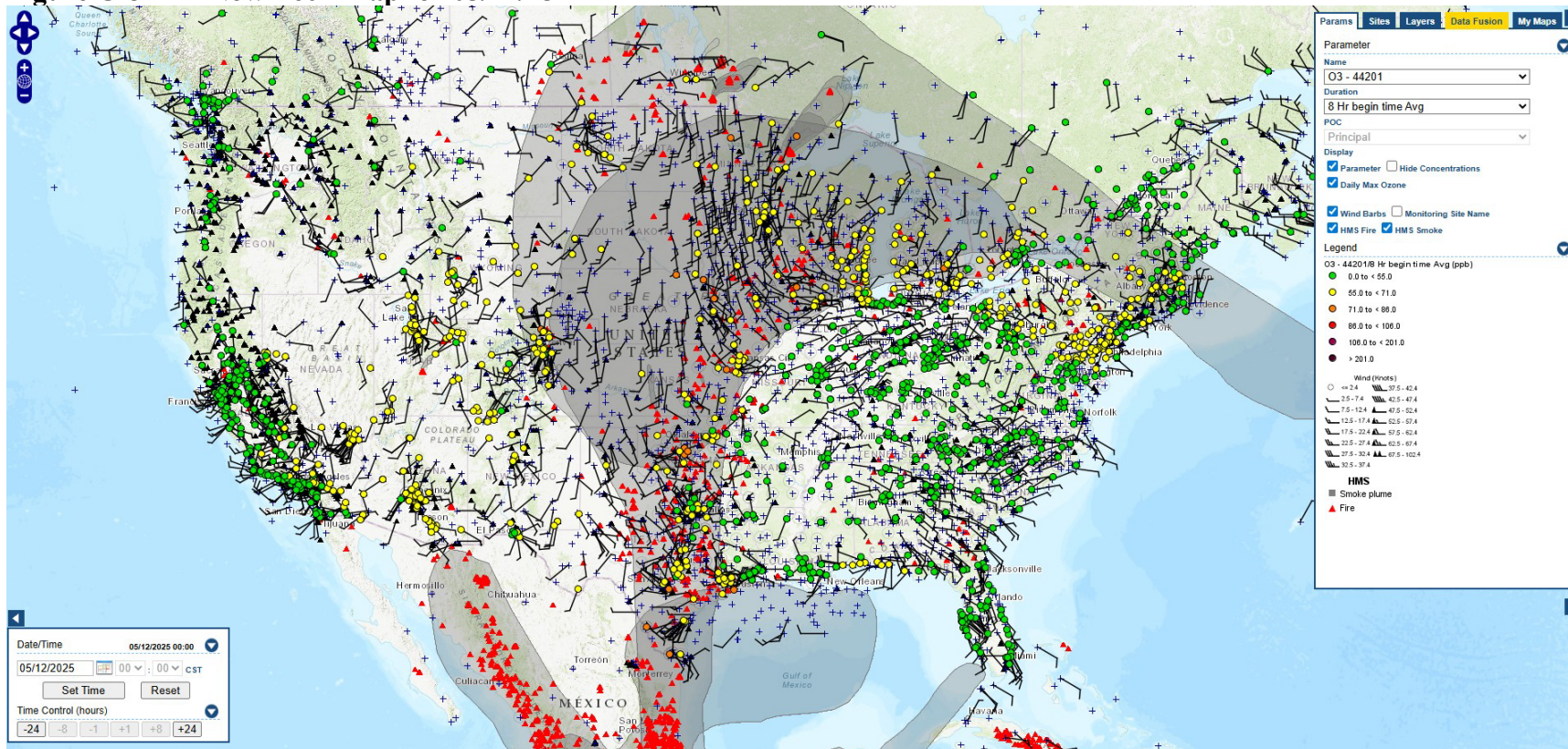
Figure C-8 - AirNow Tech Map for 05/12/25
