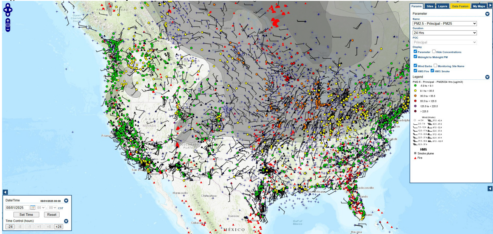
Figure A-14 – AirNow Tech Map for 08/01/25
