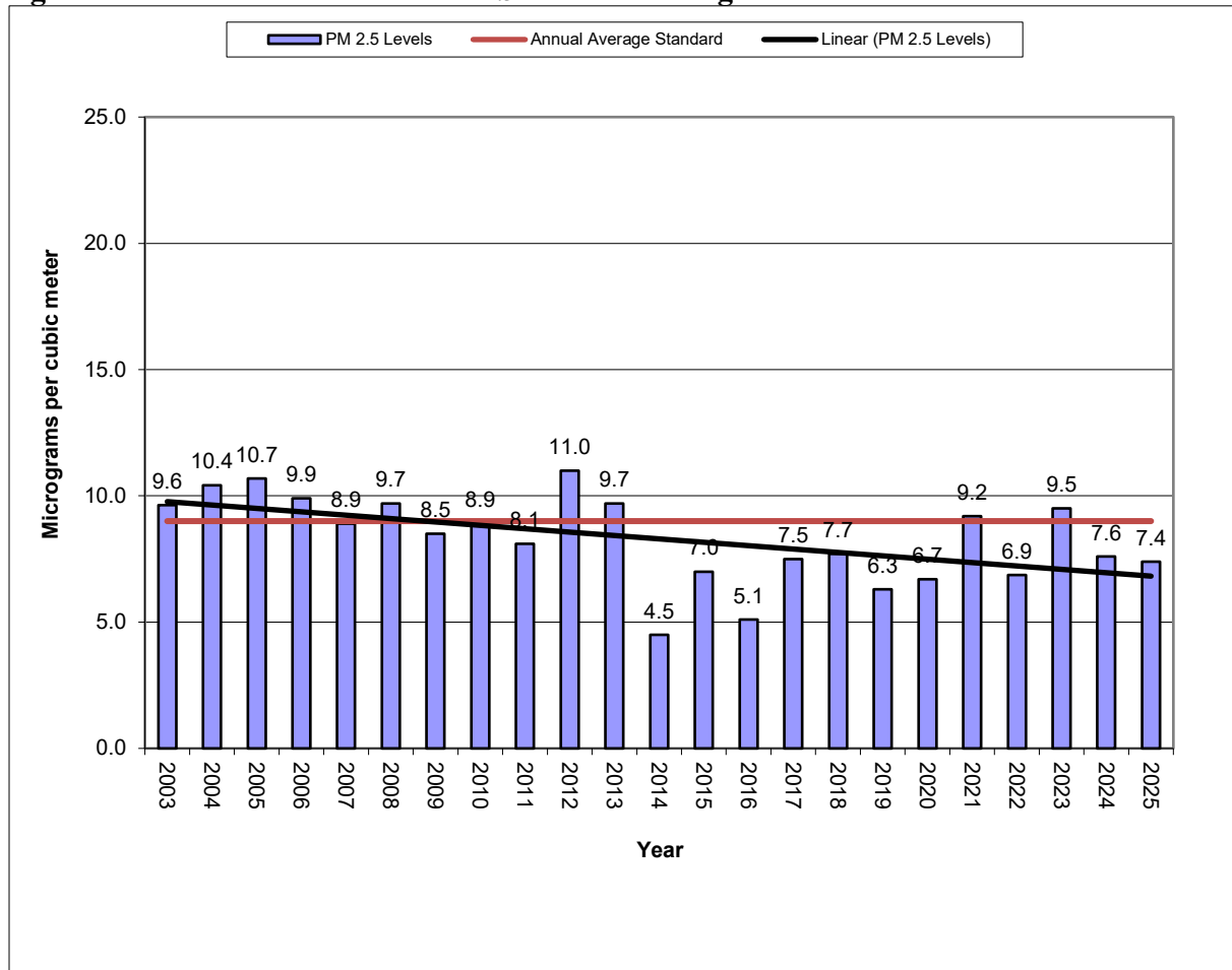
Figure 10-33 – Watertown Site PM 2.5 Annual Averages
