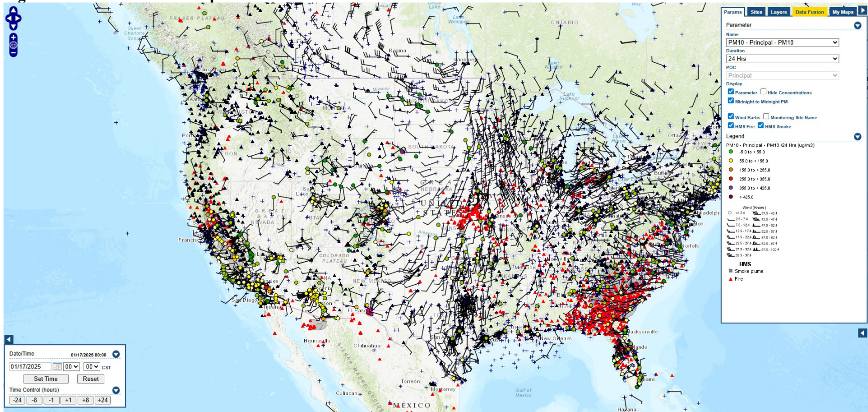
Figure B-2 - AirNow Tech Map for 01/17/25
