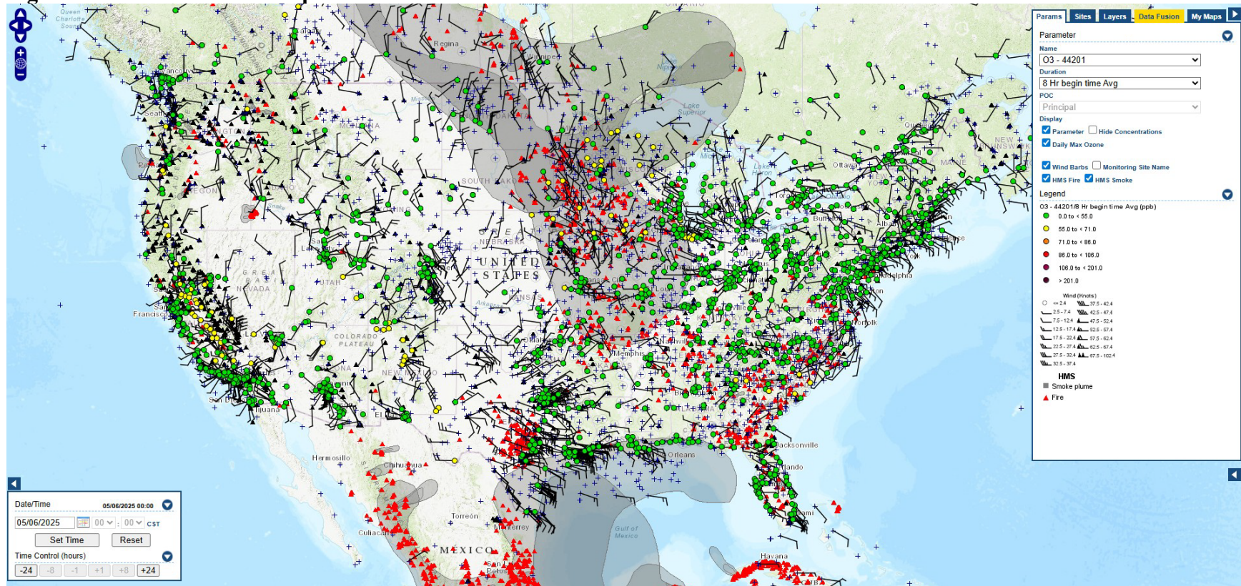
Figure C-2 - AirNow Tech Map for 05/06/25
