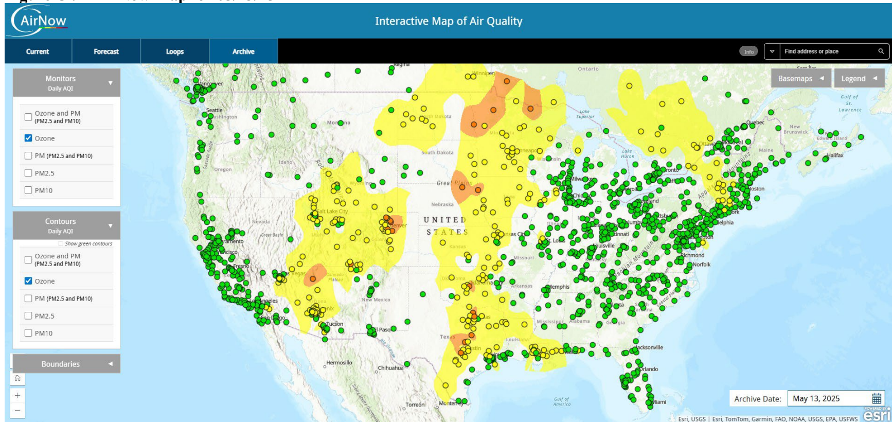
Figure C-9 - AirNow Map for 05/13/25
