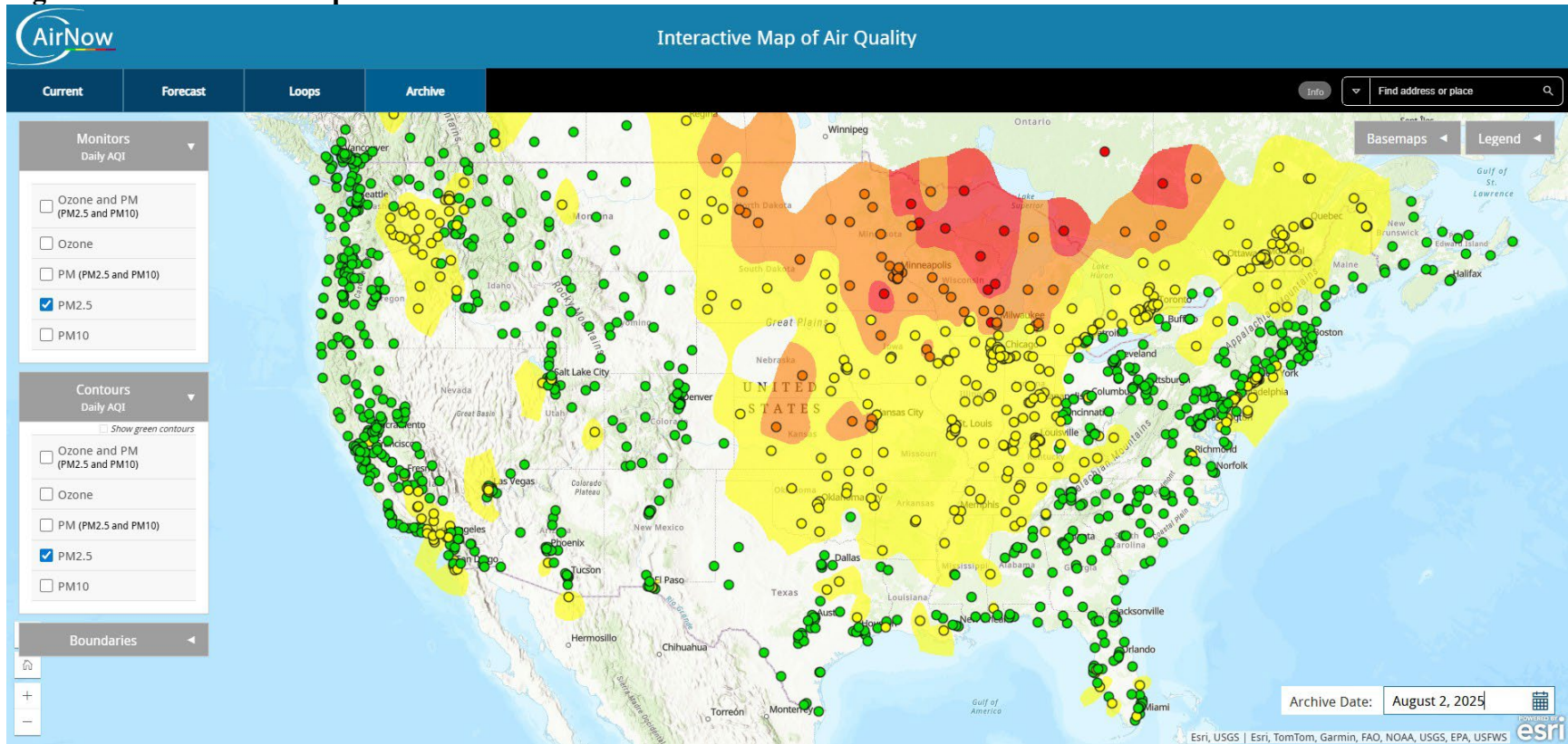
Figure A-15 – AirNow Map for 08/02/25
