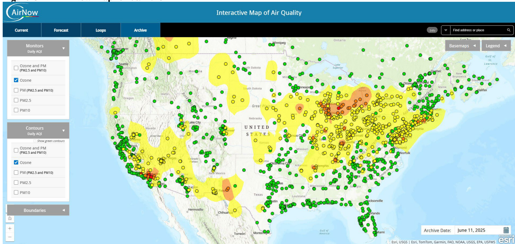
Figure C-17 - AirNow Map for 06/11/25
