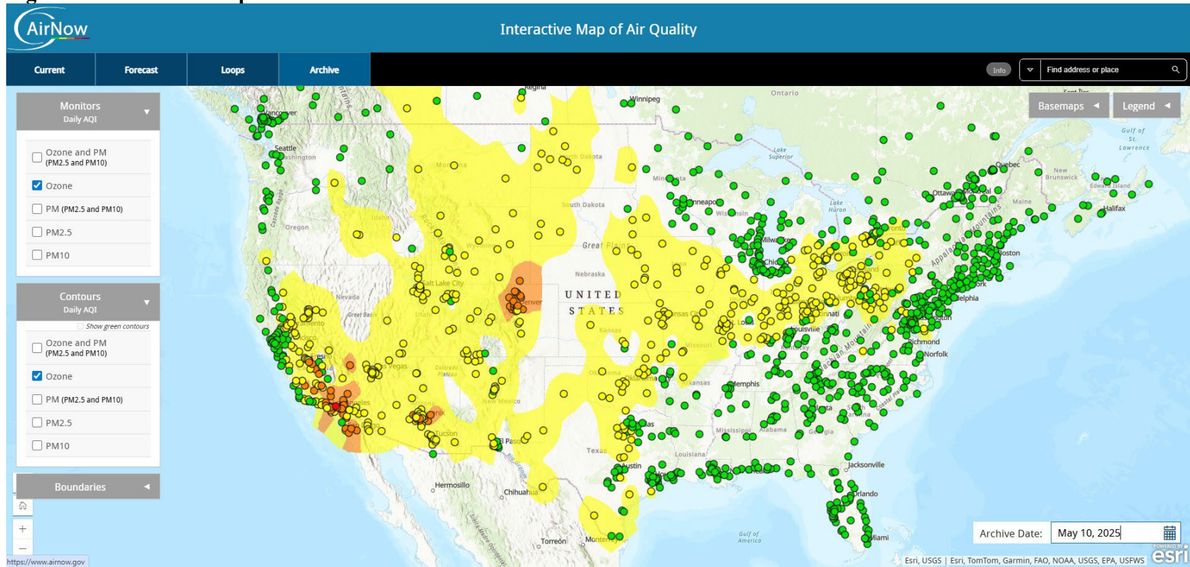
Figure C-3 - AirNow Map for 05/10/25
