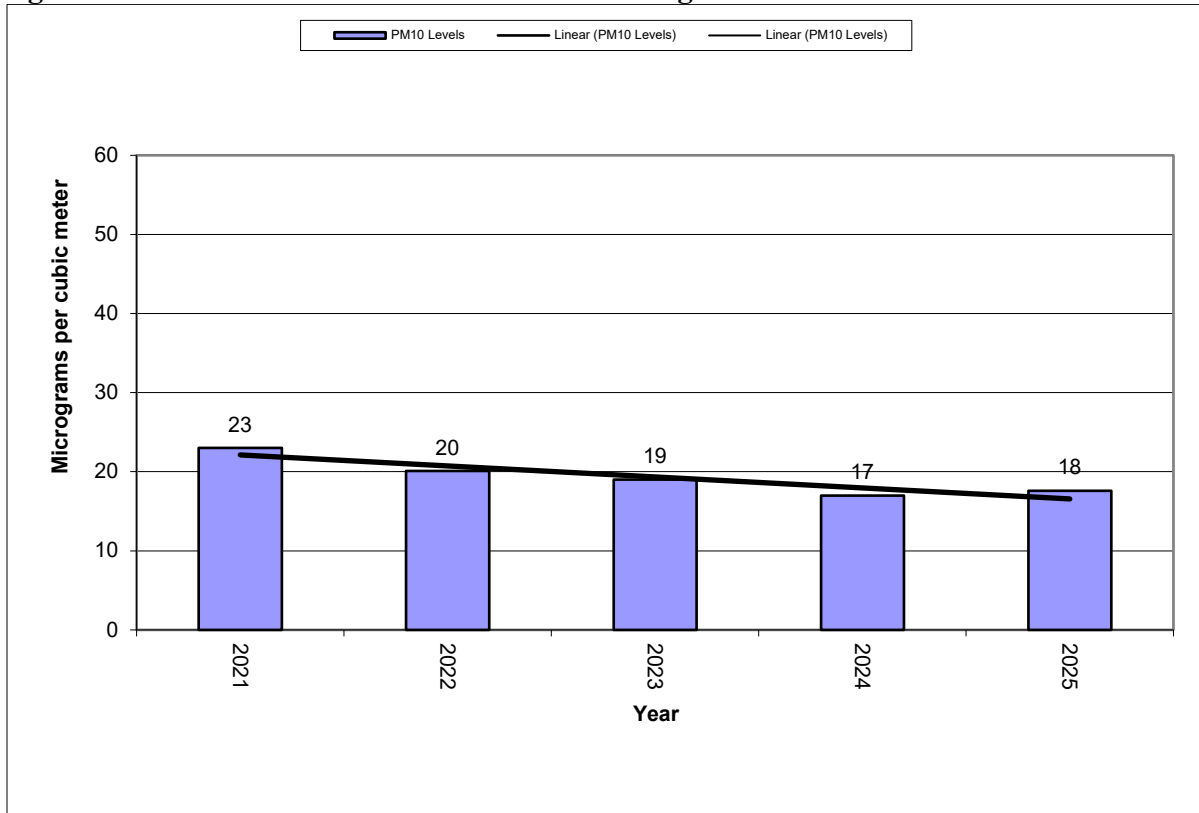
Figure 10-18 – SF USD Site – PM 10 Annual Averages
