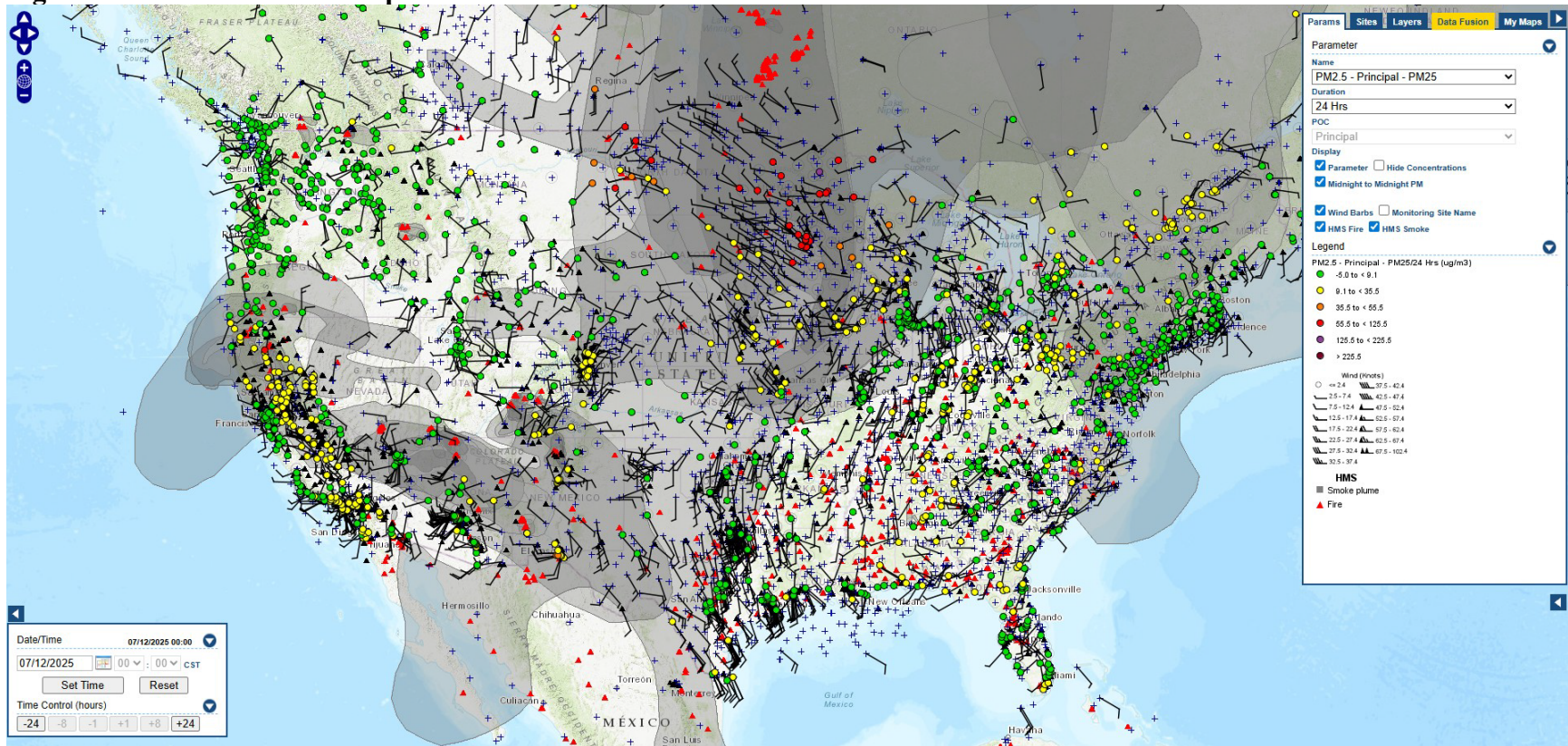
Figure A-8 – AirNow Tech Map for 07/12/25
