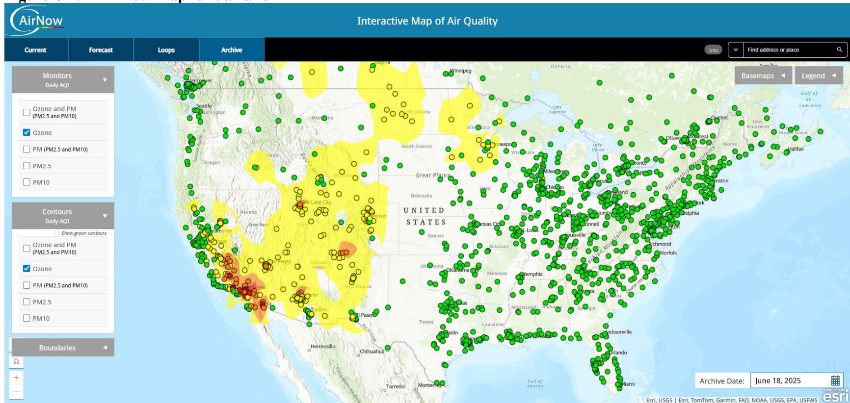
Figure C-19 - AirNow Map for 06/18/25
