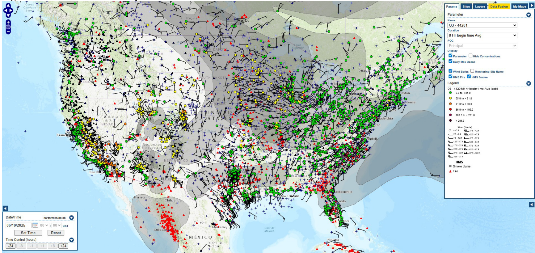
Figure C-22 - AirNow Tech Map for 06/19/25
