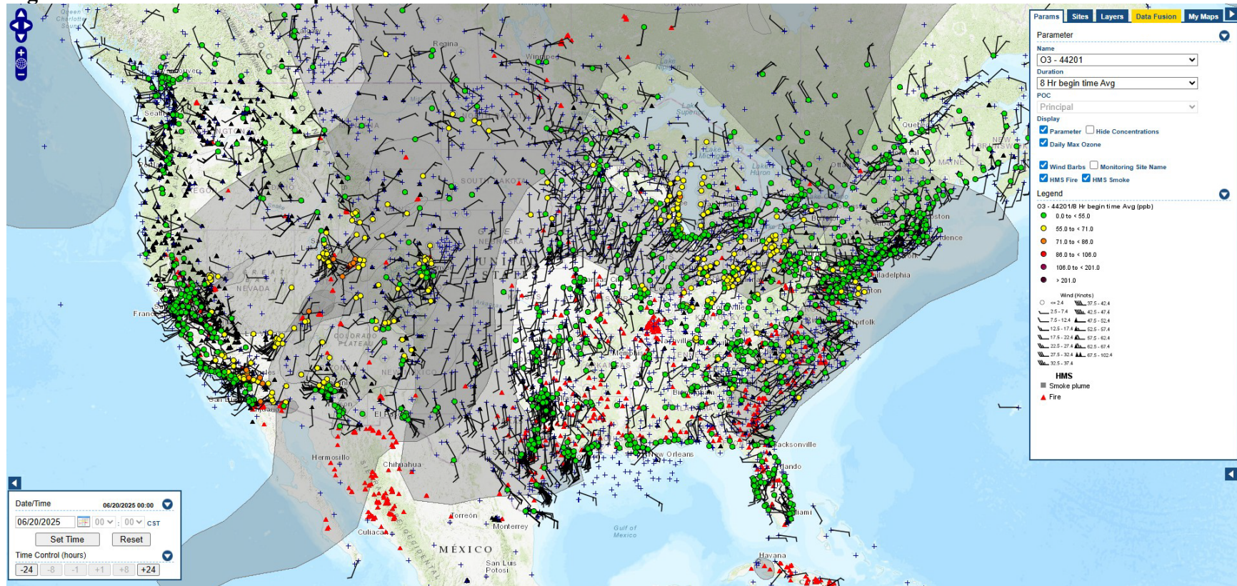
Figure C-24 - AirNow Tech Map for 06/20/25
