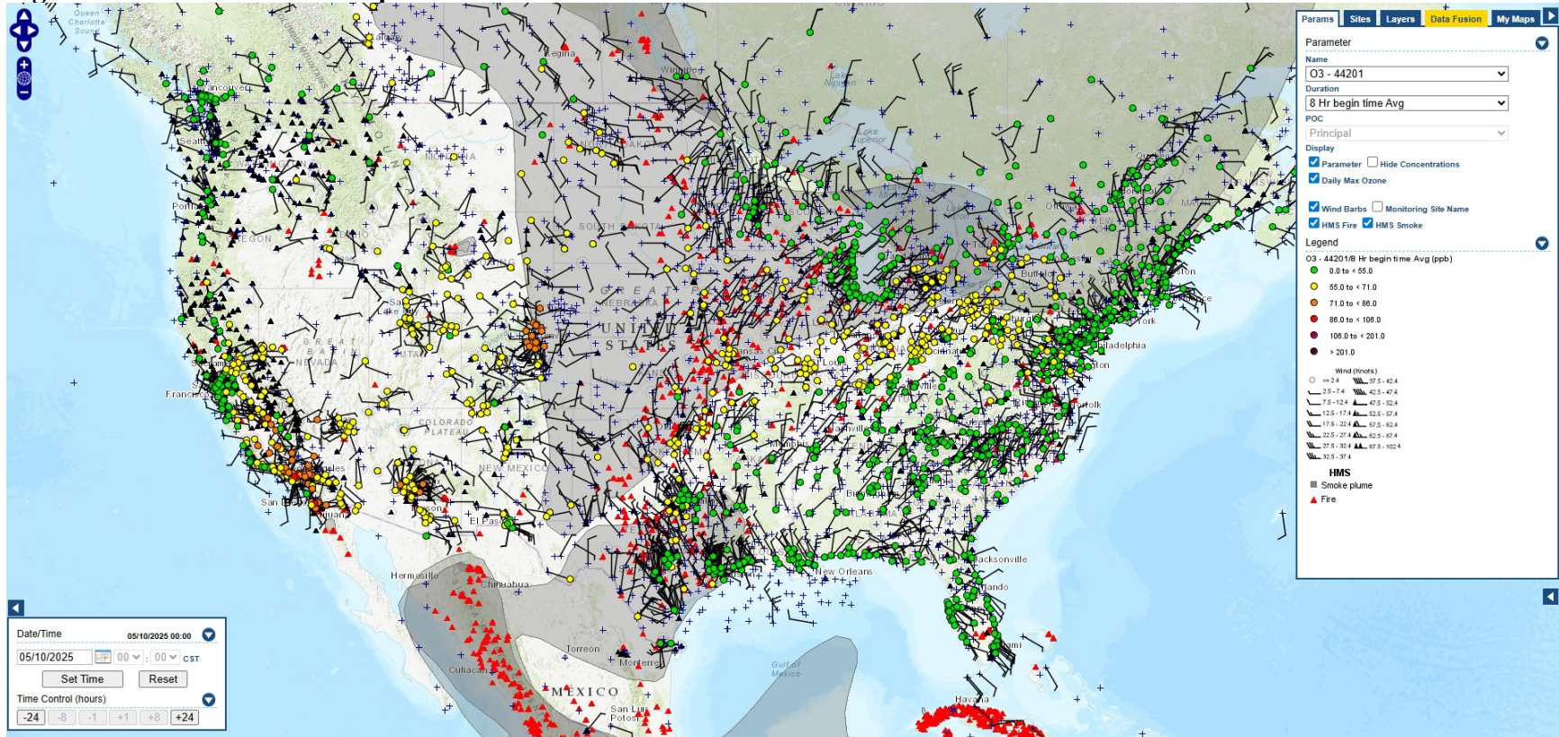
Figure C-4 - AirNow Tech Map for 05/10/25
