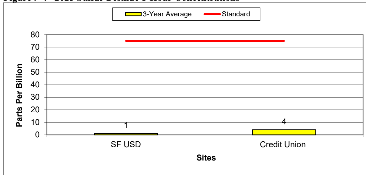
Figure 9-4– 2025 Sulfur Dioxide 1-Hour Concentrations
