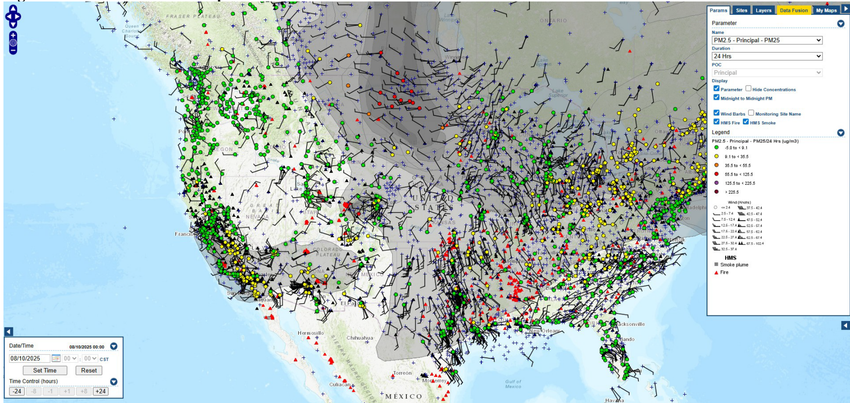
Figure A-18 – AirNow Tech Map for 08/10/25
