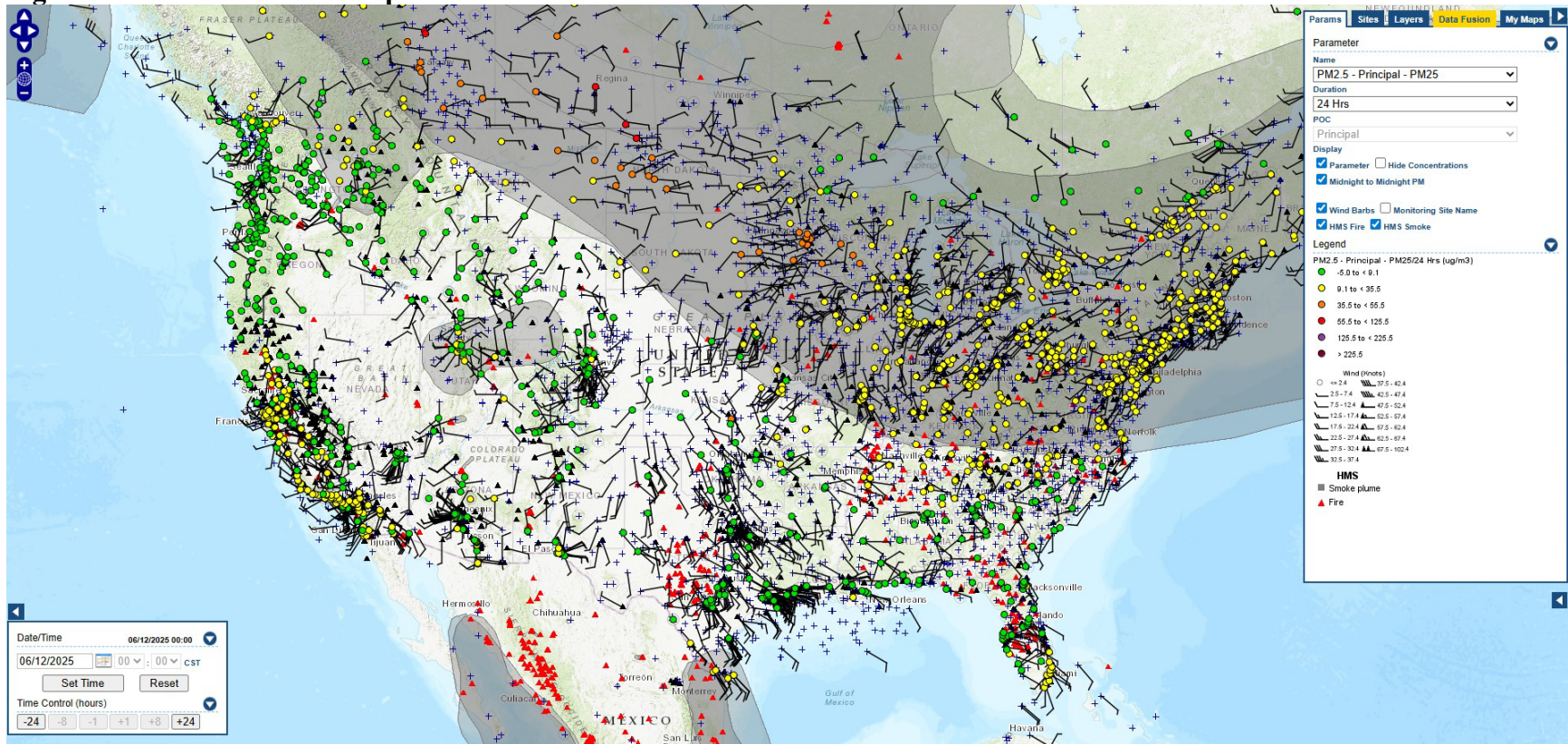
Figure A-6 – AirNow Tech Map for 06/12/25
