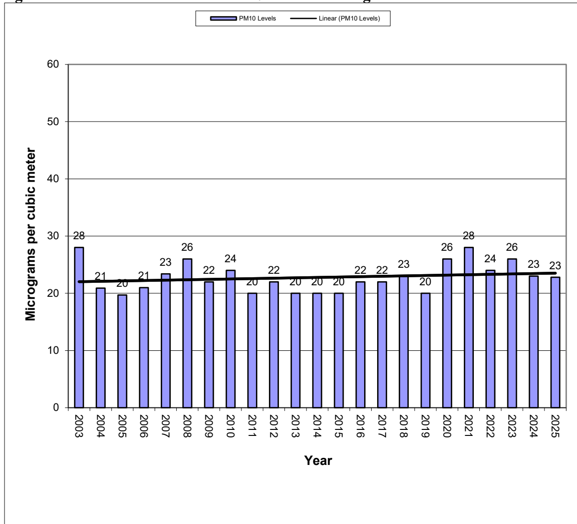
Figure 10-32 – Watertown Site – PM 10 Annual Averages
