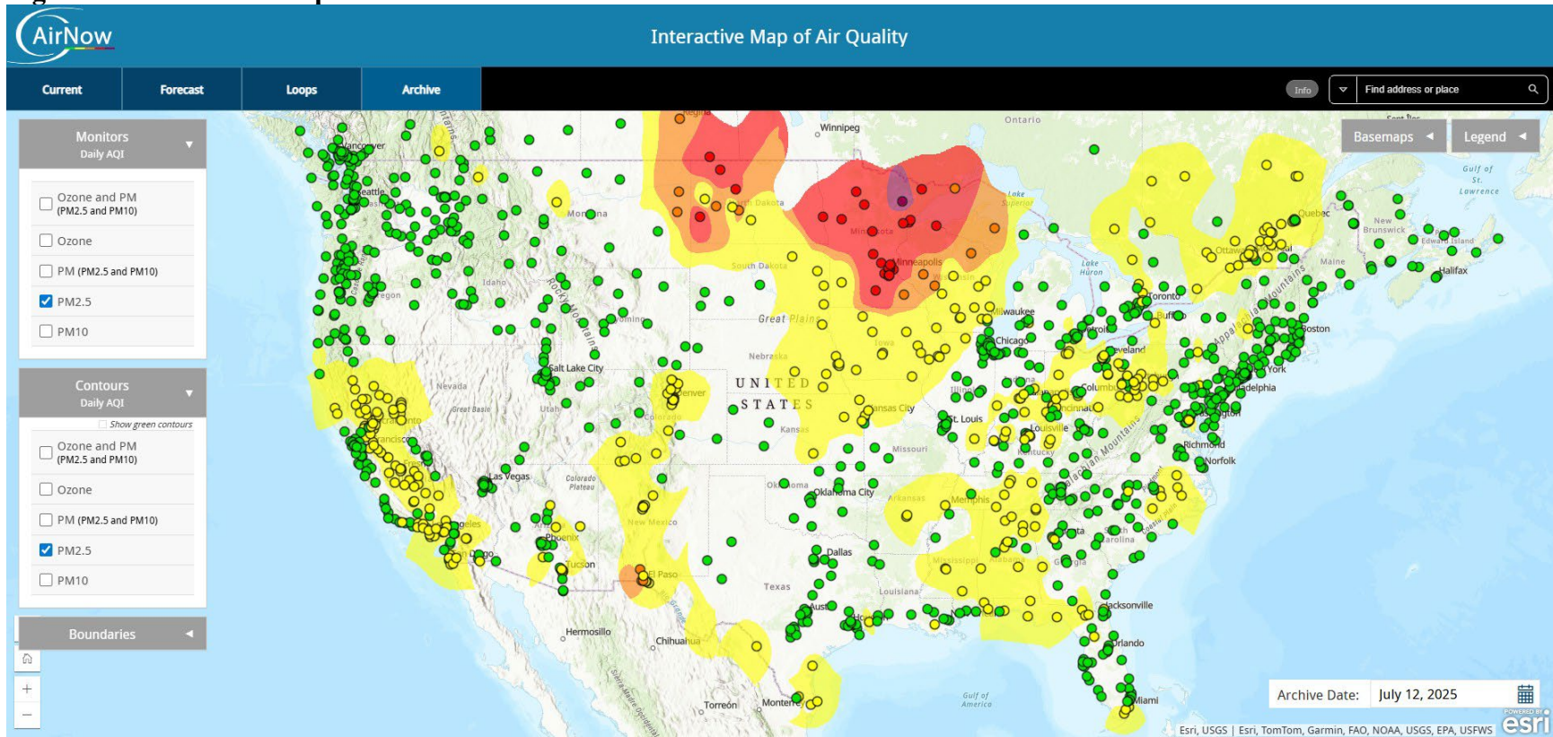
Figure A-7 – AirNow Map for 07/12/25
