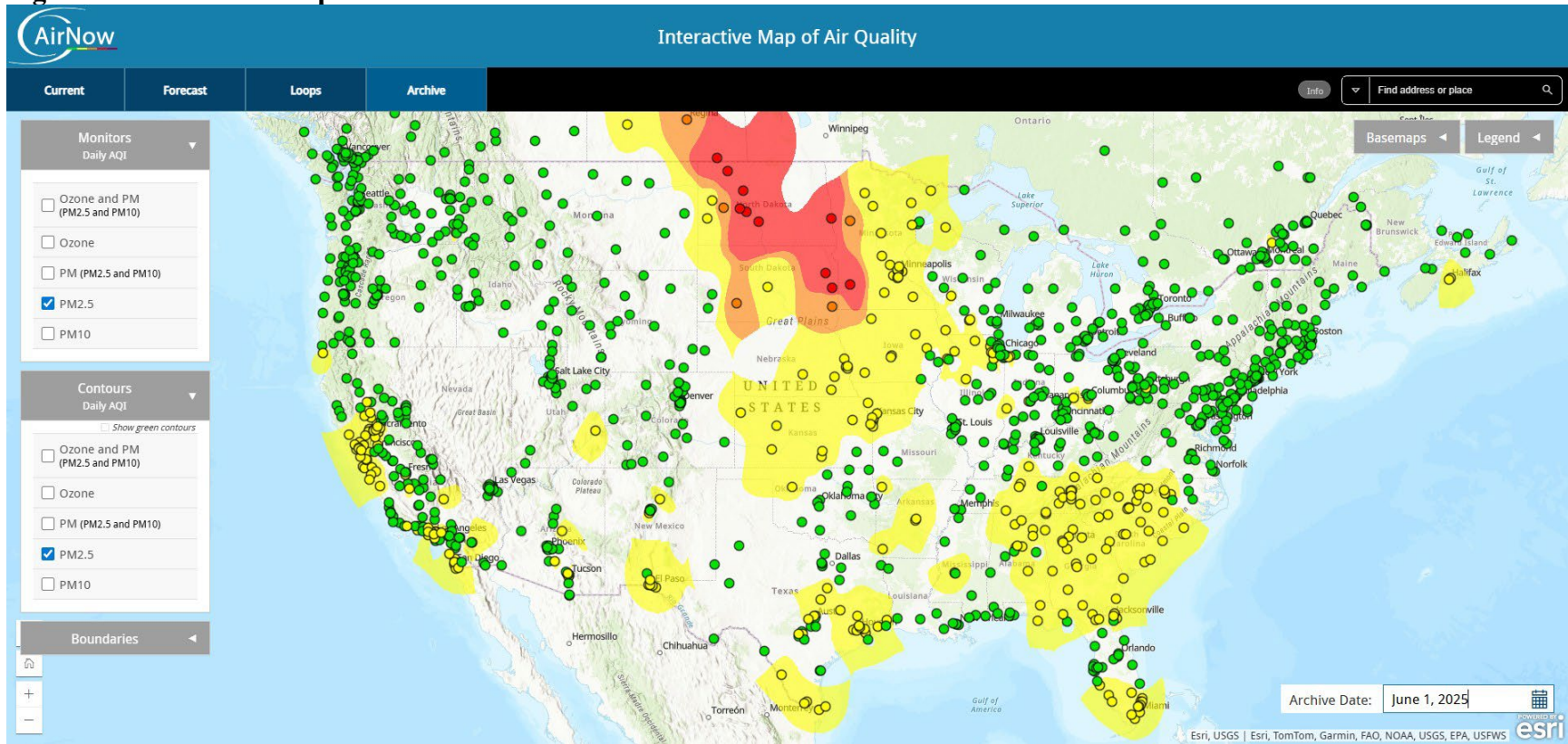
Figure A-3 – AirNow Map for 06/01/25
