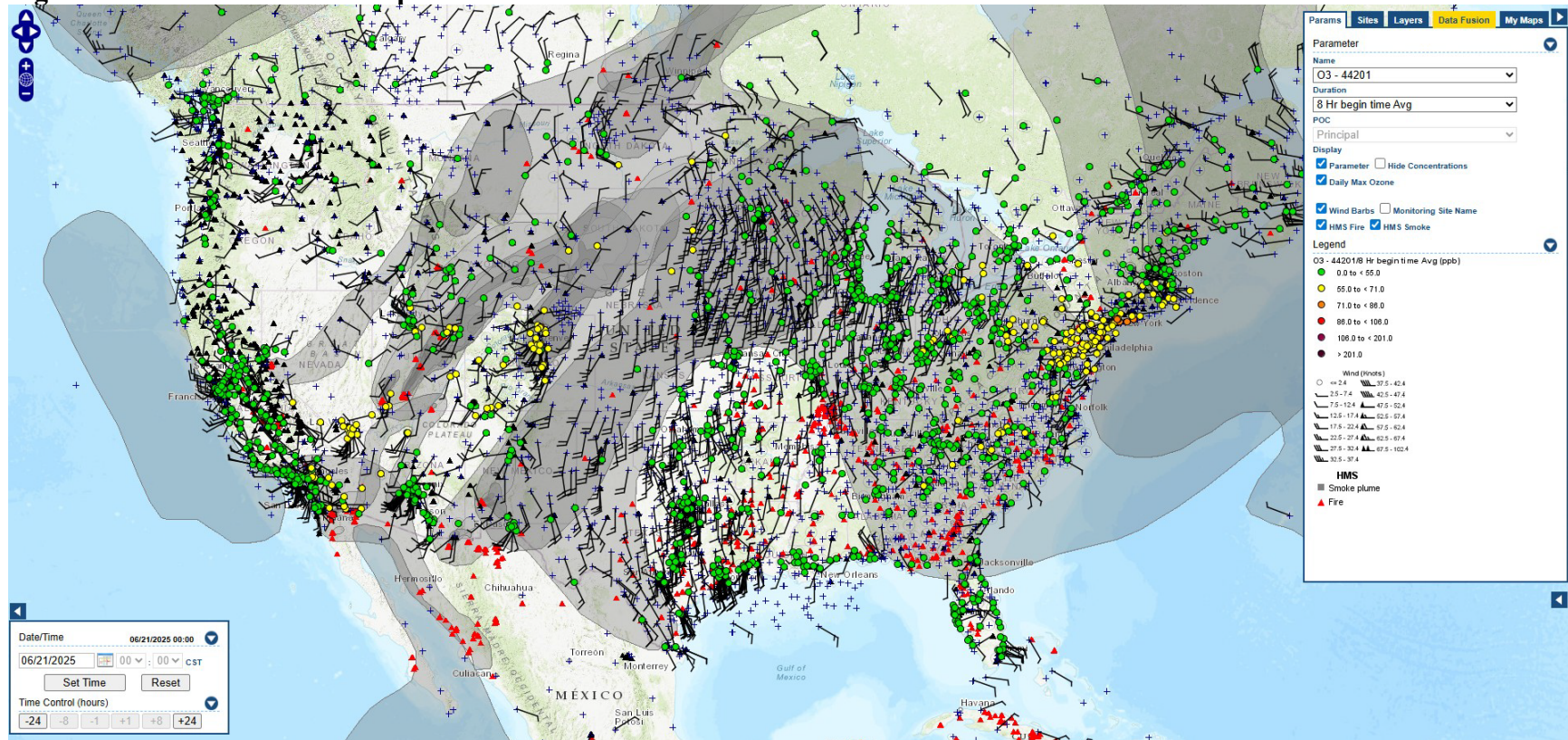
Figure C-26 - AirNow Tech Map for 06/21/25
