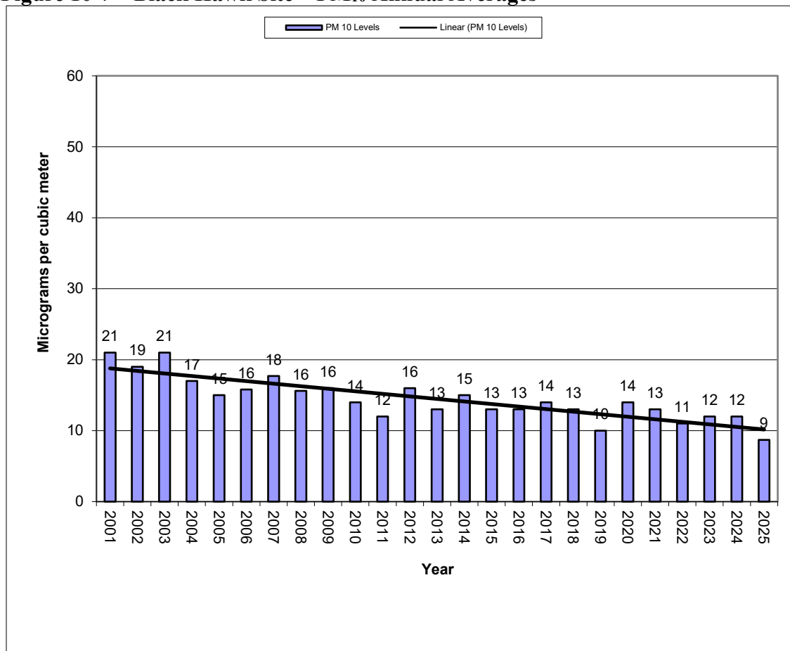
Figure 10-7 – Black Hawk Site – PM 10 Annual Averages
