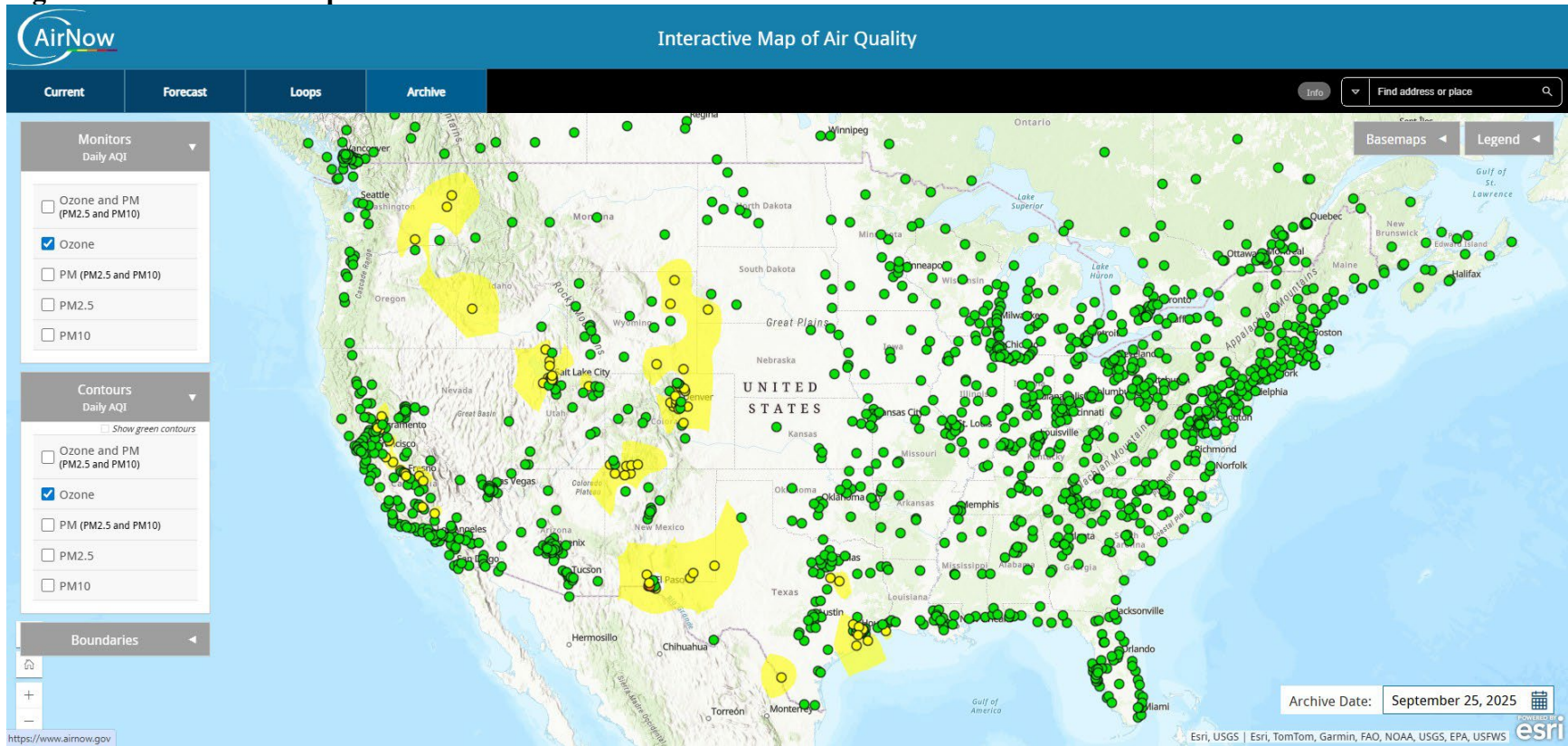
Figure C-27 - AirNow Map for 09/25/25
